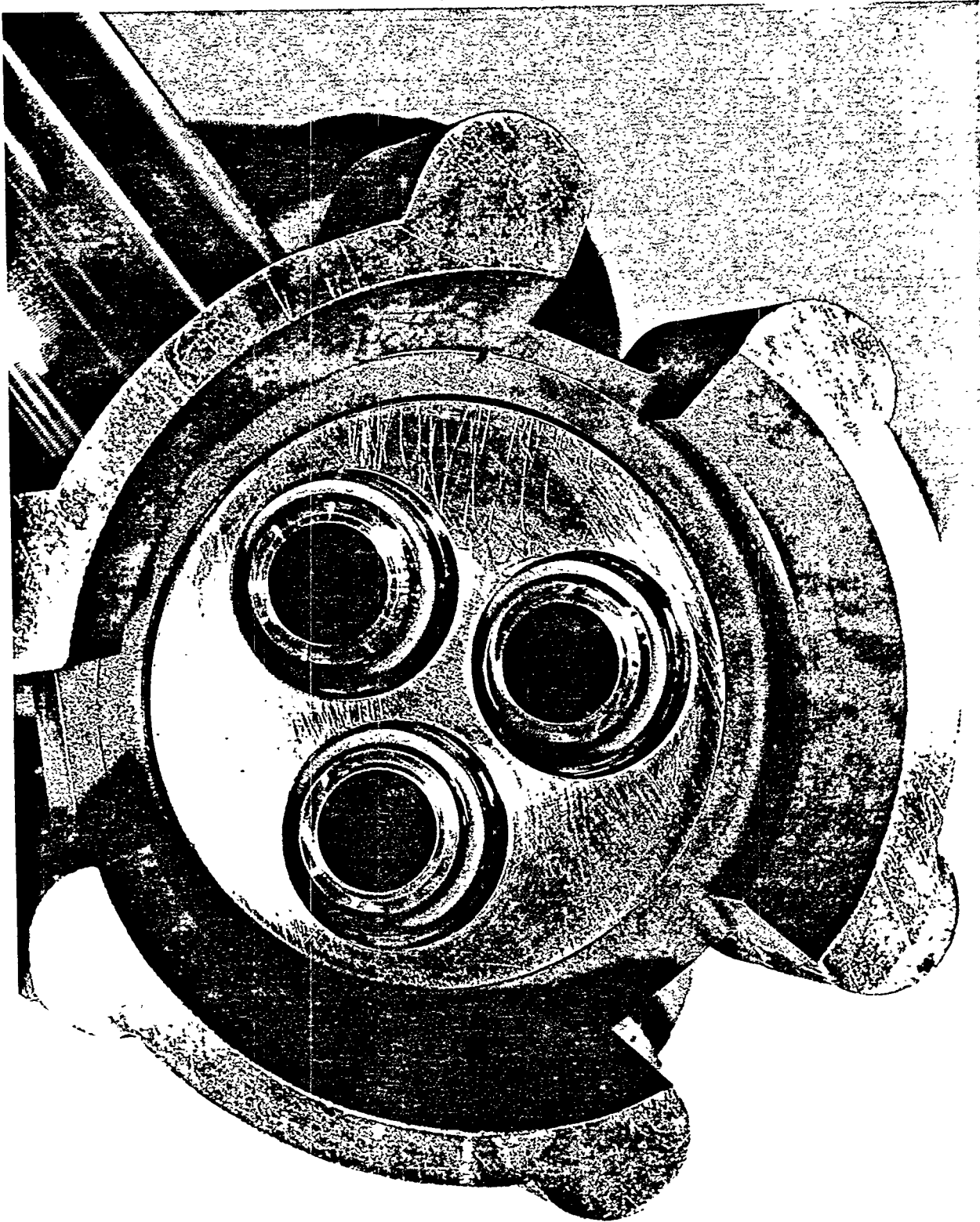
Photograph 6. Closeup View of Three-Way Integral Seal Block Installed in Vertical Skirt, Showing O-Ring Seals.
