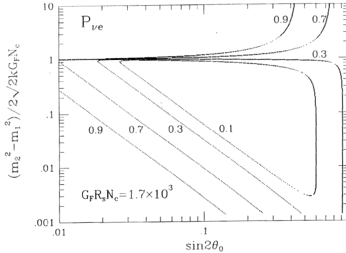
FIG. 1: Probability-contour plot for detecting an electron neutrino at the Earth which was produced in the solar interior.
