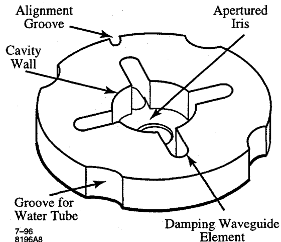
Figure 5. A cell of the Damped-Detuned structure.
