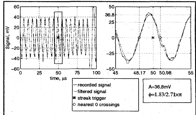
Figure 4. Extracting the instability phase and amplitude from the detector signal
