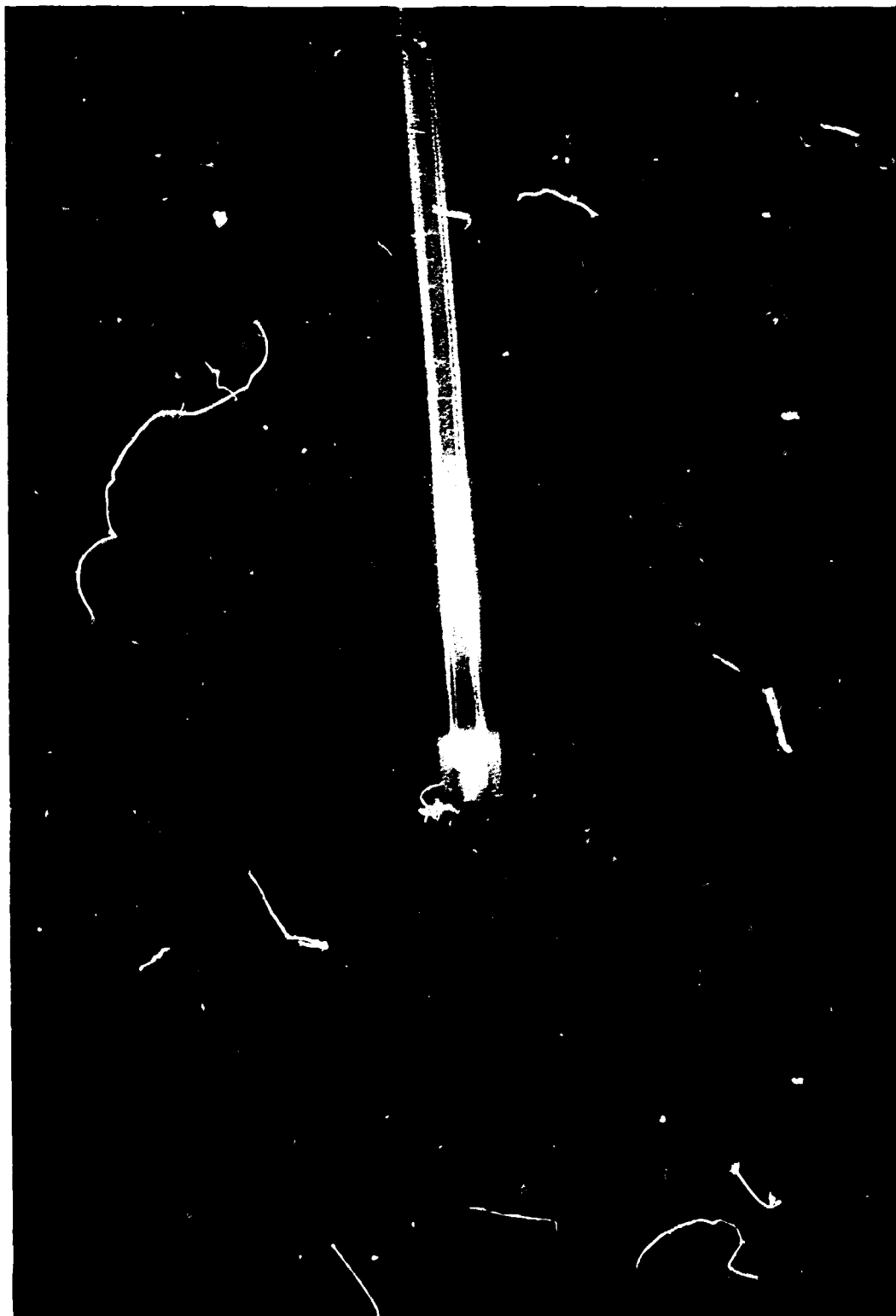
Figure 4. Radiograph of PRT S/N 3670 in the thermowell shows the relation of the silver bushing to the reduced section of thermowell.
