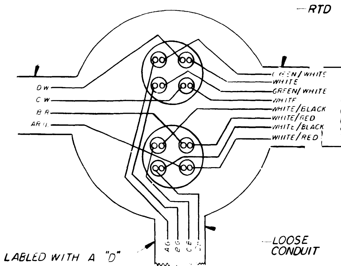
RTD WIRING FIGURE 7a
