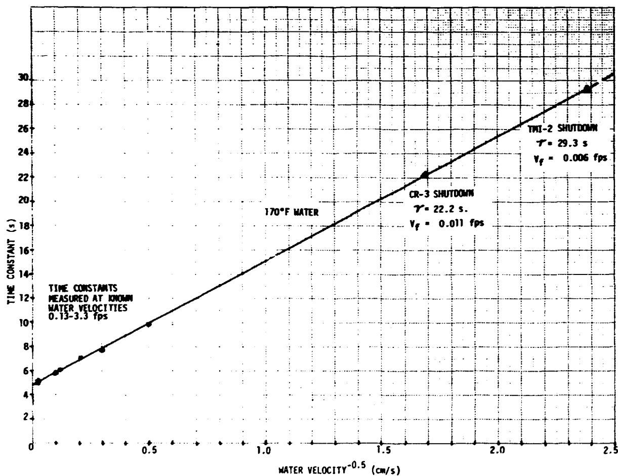
Figure 8. Estimates of still/natural circulation water flow velocities from PRT time response measured during shutdown in TMI-2 and CR-3.
