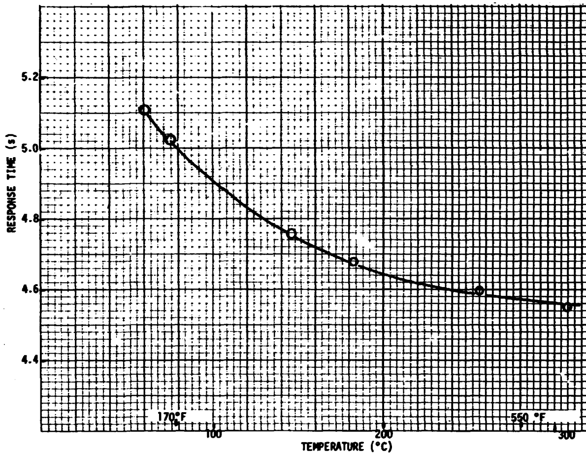
Figure 9. Temperature dependence of response time of REC Model 177 HW PRT in thermowell when measured in GIT. (Equivalent to water at 170°F.)
