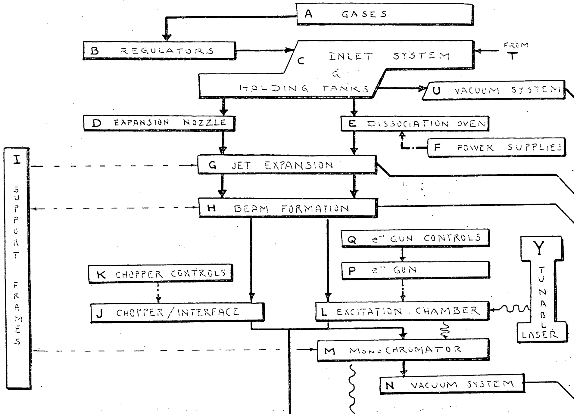
BLOCK DIAGRAM
