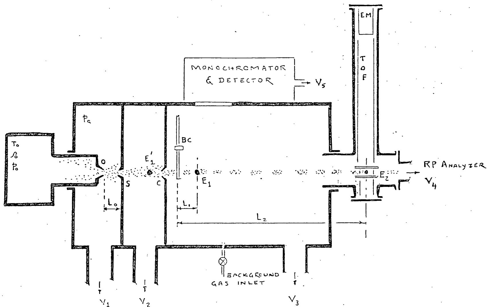
Figure 2. Experimental Apparatus
