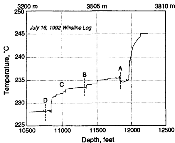
Fig. 1. A typical temperature profile across the Production Interval
