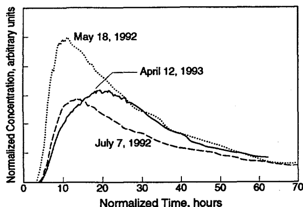
Fig. 4. Recovery of fluorescein dye tracer on three occasions; early and late during the 8-months of flow testing in 1992, and 4 weeks after renewed flow testing in 1993
