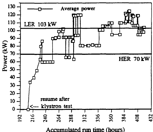
Figure 3. Phase 1 cavity test processing history, part 2.
