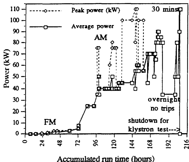
Figure 2. Phase 1 cavity test processing history, part 1.
