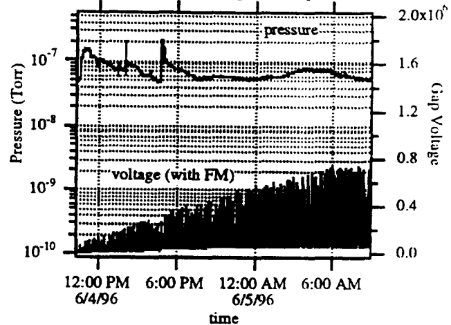
Figure 5. Recorded data from automated RF processing with FM after a controlled vent.
