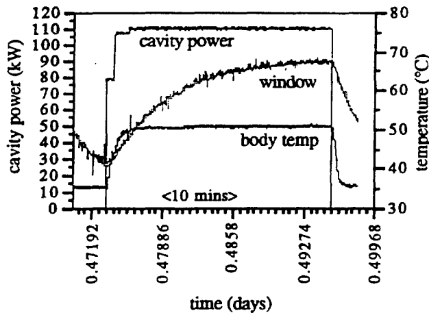
Figure 4. Window and body temperature at high power.
