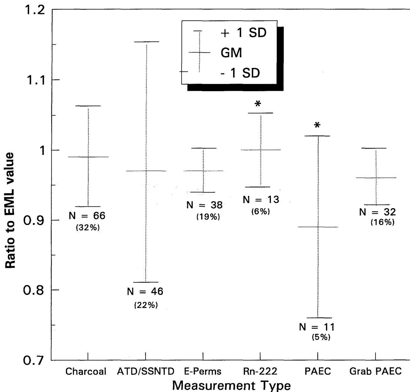
Figure 6. Data summary of 5th Radon/Progeny Intercomparison.
