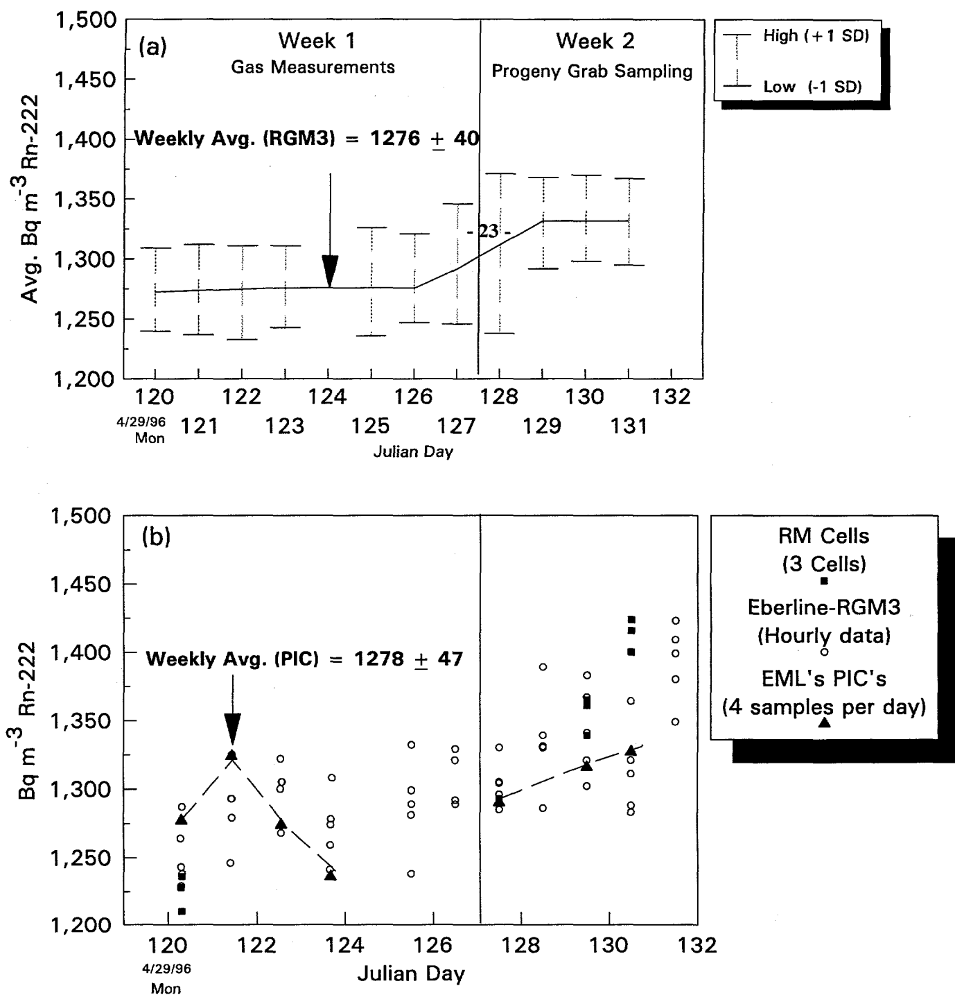
Figure A1. 222 Rn data. (a) daily Averages in EML radon chamber using Eberline RGM3 scintillation cell. (b) data during random grab sampling using EML's PICs and RM scintillation cells.
