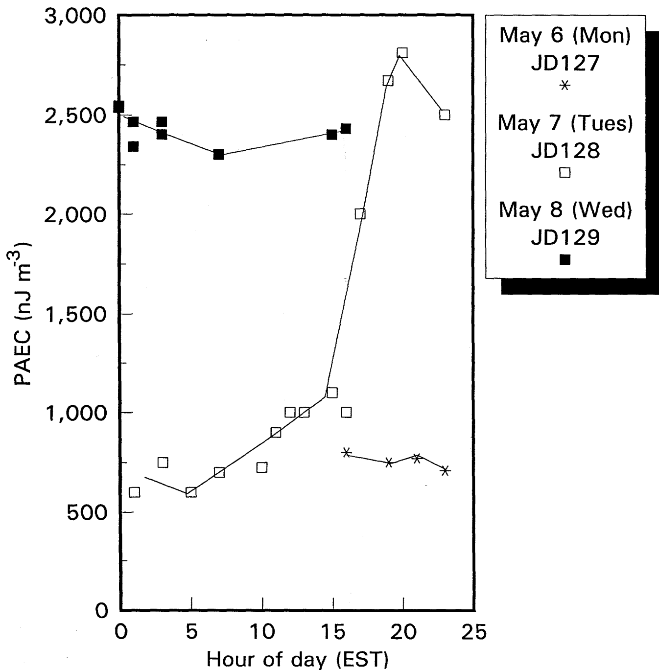
Figure A2. Radon progeny data summary during grab sampling. Alpha Nuclear Smart-770; JD = Julian day #.
