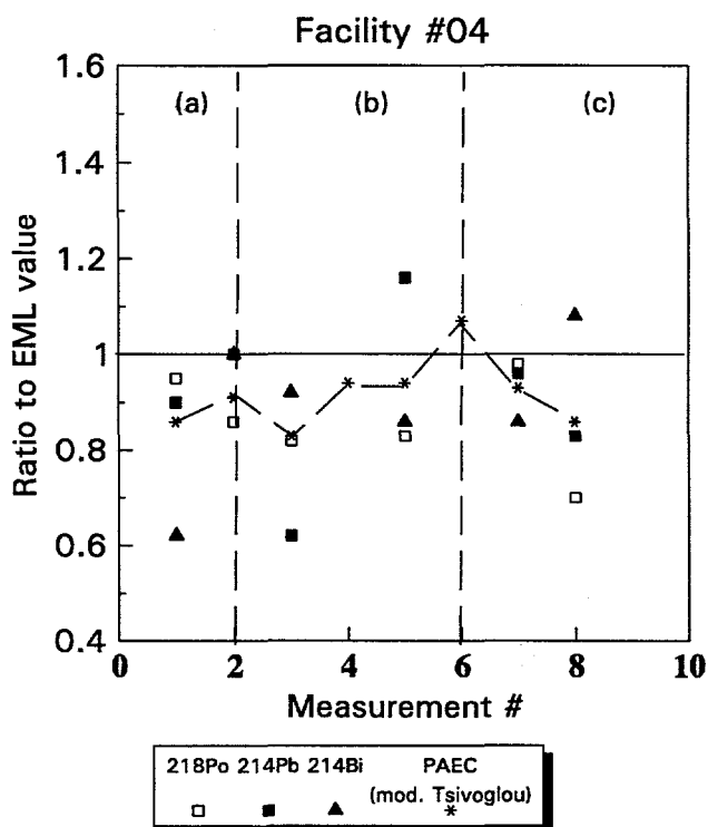
Figure 3. Results of 5th Radon/Progeny Intercomparison: Grab Sampling:
