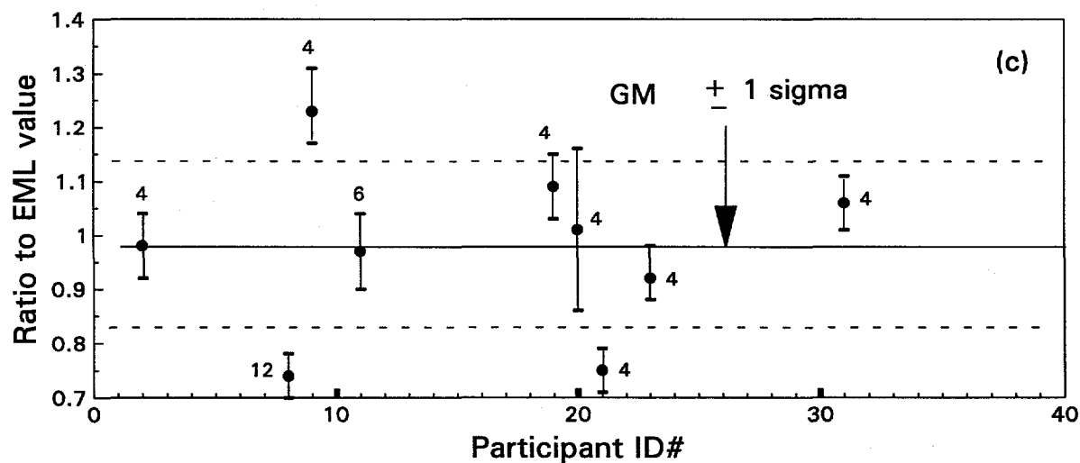
Figure 1. Results of 5th Radon/Progeny Intercomparison. Passive Radon-222 devices: (a) activated charcoal; (b) E-Perms; (c) ATDs/SSNTDs ;
