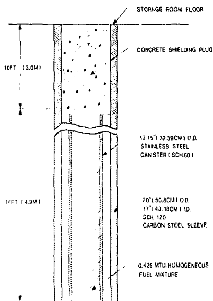
Fig. 2: Emplacement package details.
