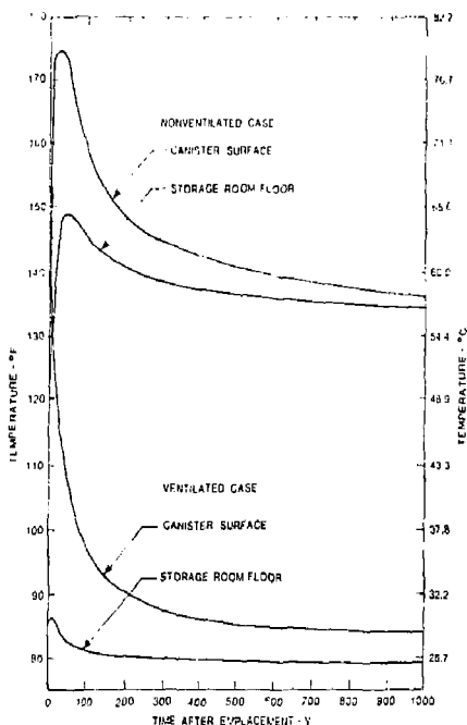
Fig. 4: Canister surface and storage room floor temperature histories for both ventilated (with 79°F air at 10,000 CPM) and unventilated cases.
