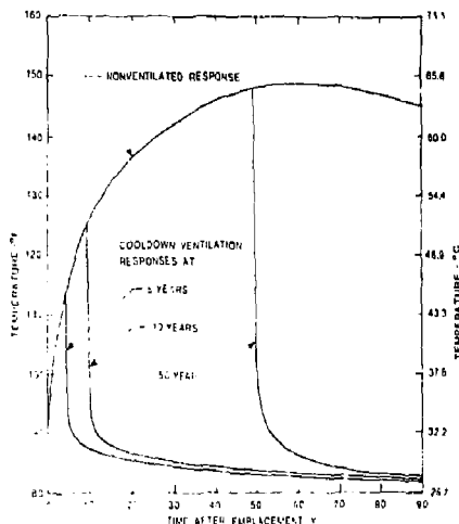
Fig. 5: Storage room floor temperature histories representing cool-down (10,000 CFM of air) from an unventilated state at 5, 10, and 50 years.
