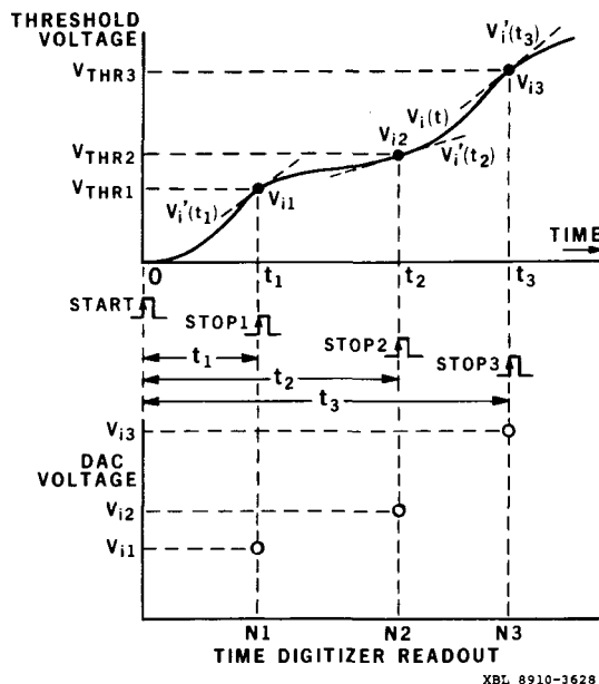
Fig. 1 Procedure for reconstruction of a measured waveform by plotting comparator threshold crossing time.
