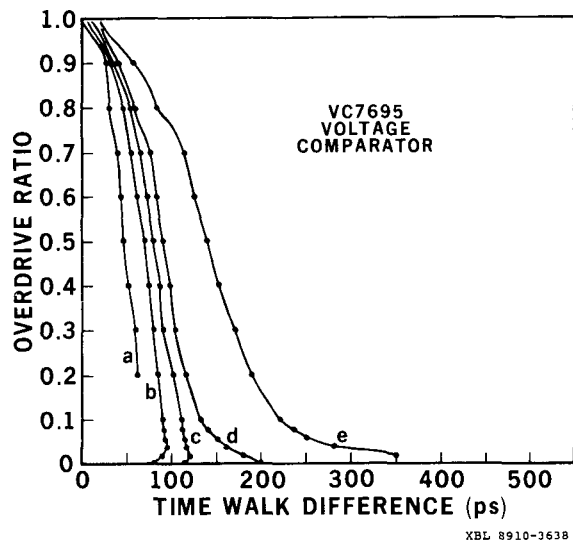
Fig. 11 Compensation of normalized time walk of VC7695 (Fig. 7) by subtracting the input pulse leading edge time.
