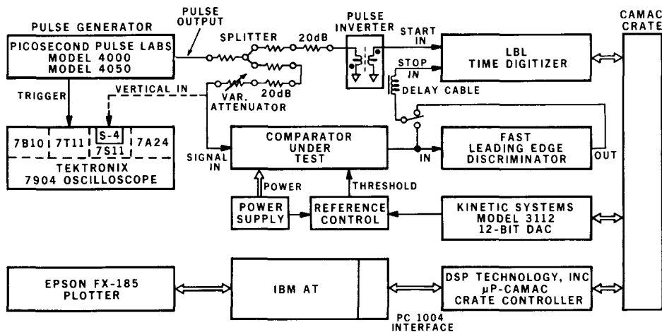
Fig. 3 Block diagram of the measurement system.
