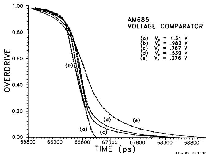
Fig. 9 Normalized time walk of AM685 comparator.
