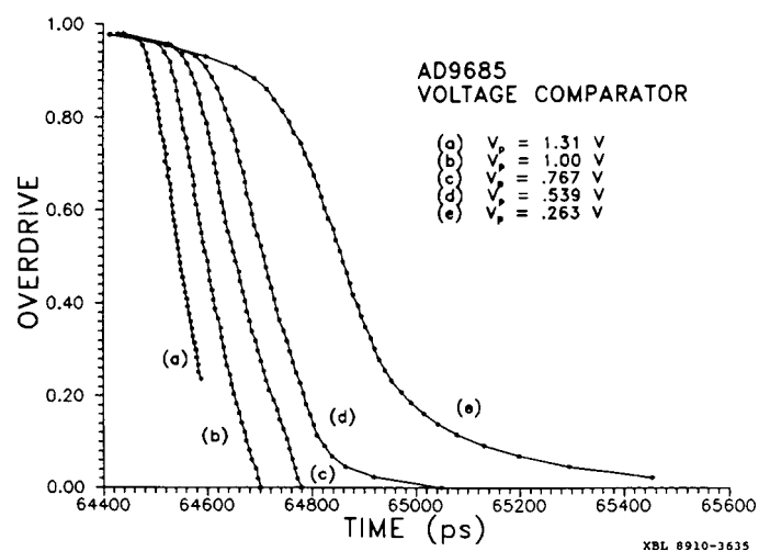
Fig. 8 Normalized time walk of AD9685 comparator.
