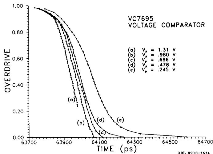
Fig. 7 Normalized data from Fig. 6 showing comparator time walk as function of overdrive ratio
