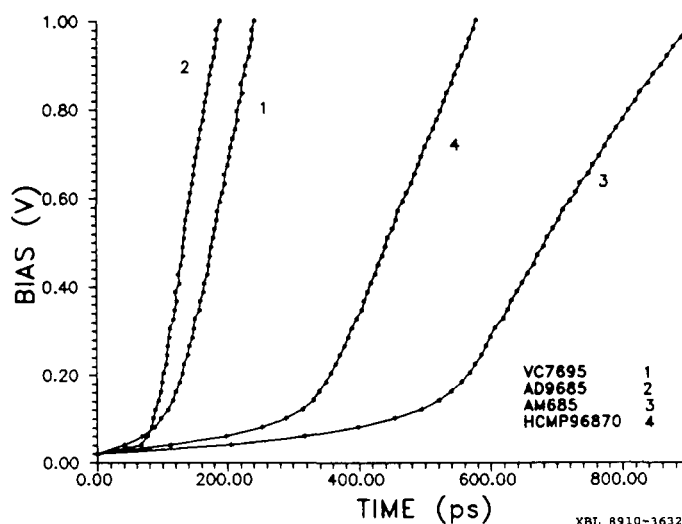
Fig. 5 Response of four bipolar fast comparators to 1.4 V, 120 ps rise time pulses. The curves are shifted horizontally to compensate for propagation delay differences.
