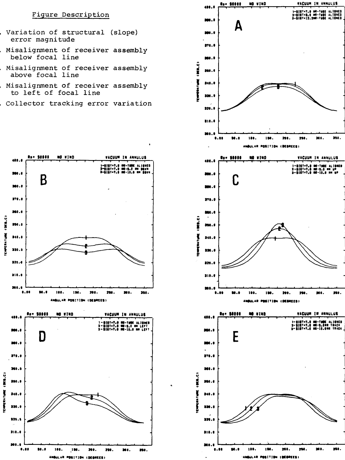
FIGURE 8. Circumferential Temperature Distributions at the Receiver Tube Surface - Re = 50,000 , Annular Space Evacuated and No Wind Velocity
