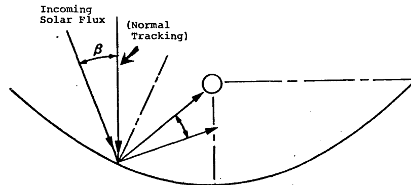
Error Associated with Tracking Bias
