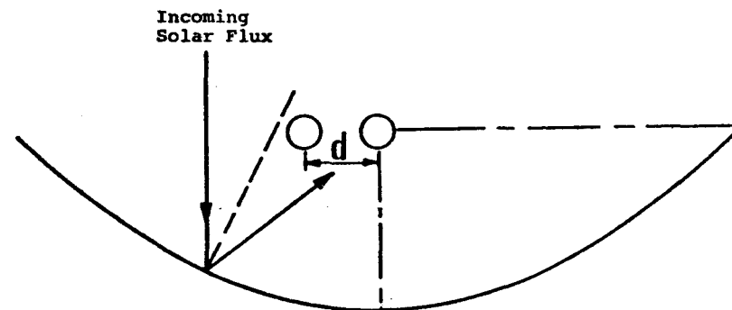
Horizontal Misalignment of the Receiver Assembly
