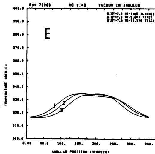
Figure A-3. Circumferential Distributions with Annular Space Evacuated-Trough Tracking Error Varied
