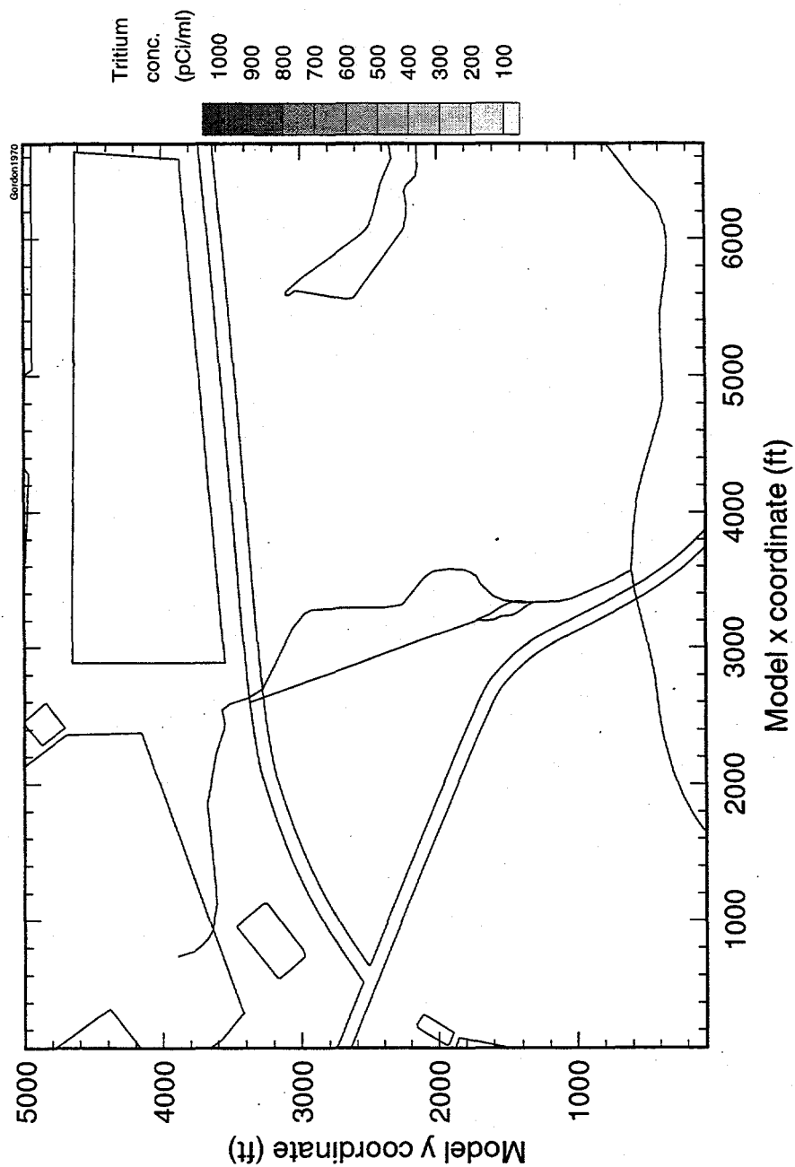
Figure 58c. Contour plot of predicted Gordon aquifer tritium concentration for 1970.
