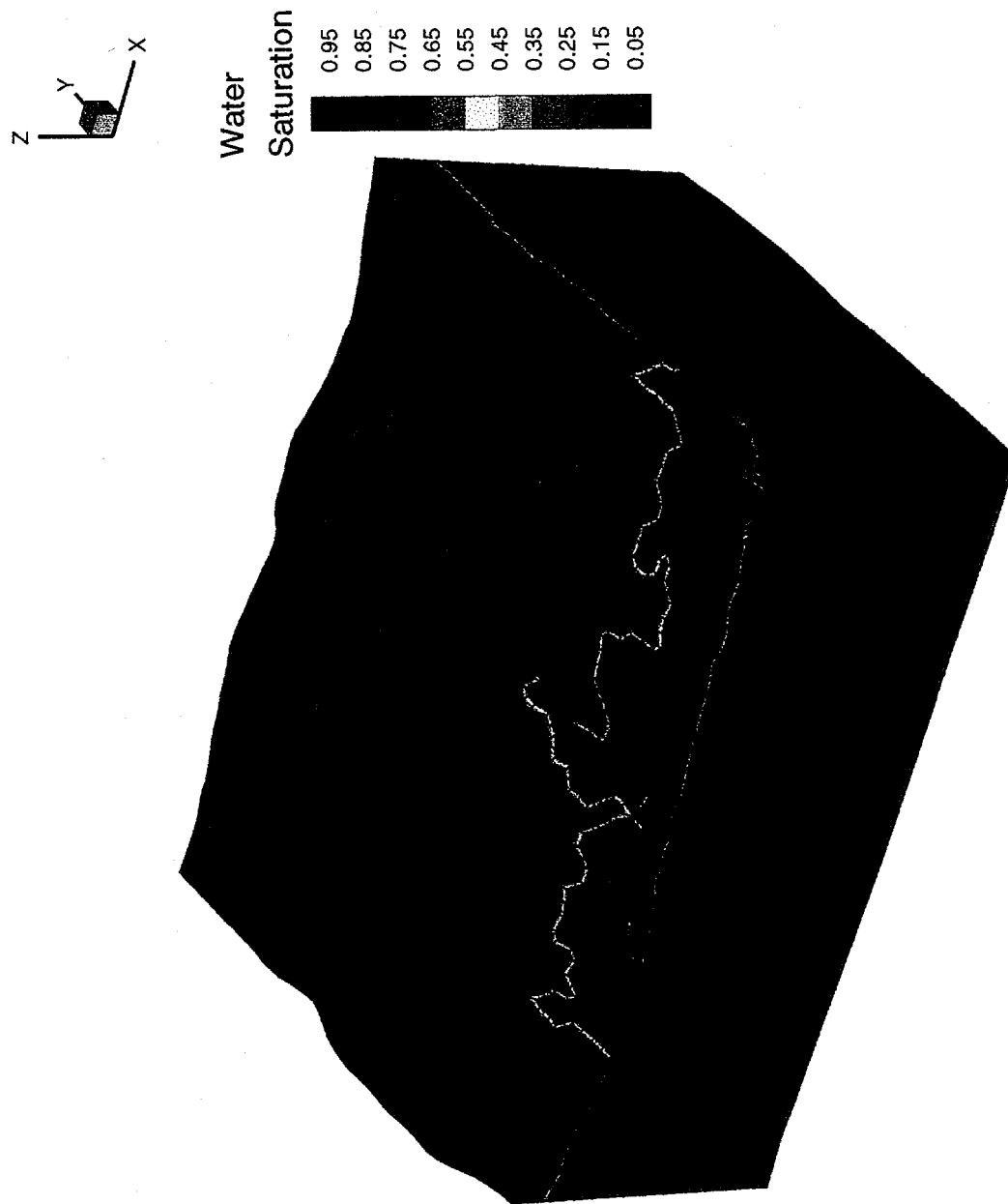
Figure 33. Simulated three-dimensional saturation distribution.
