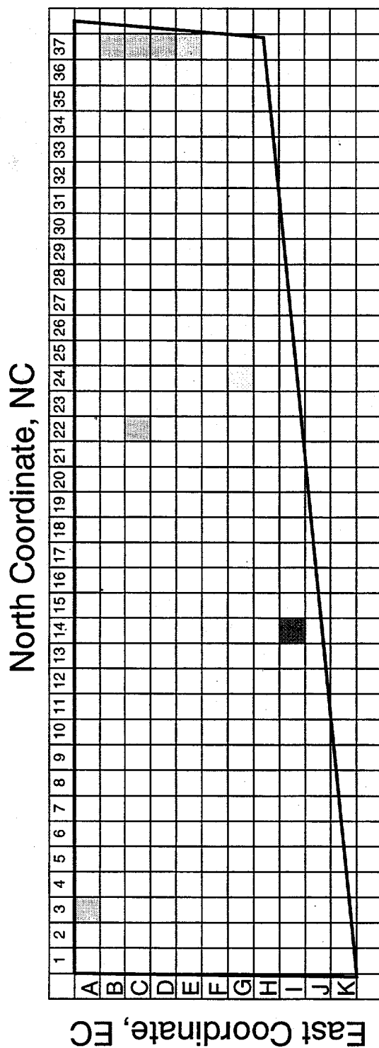
Figure 39a. Normalized spatial variation in tritium burials of all forms for the calendar year 1961.
