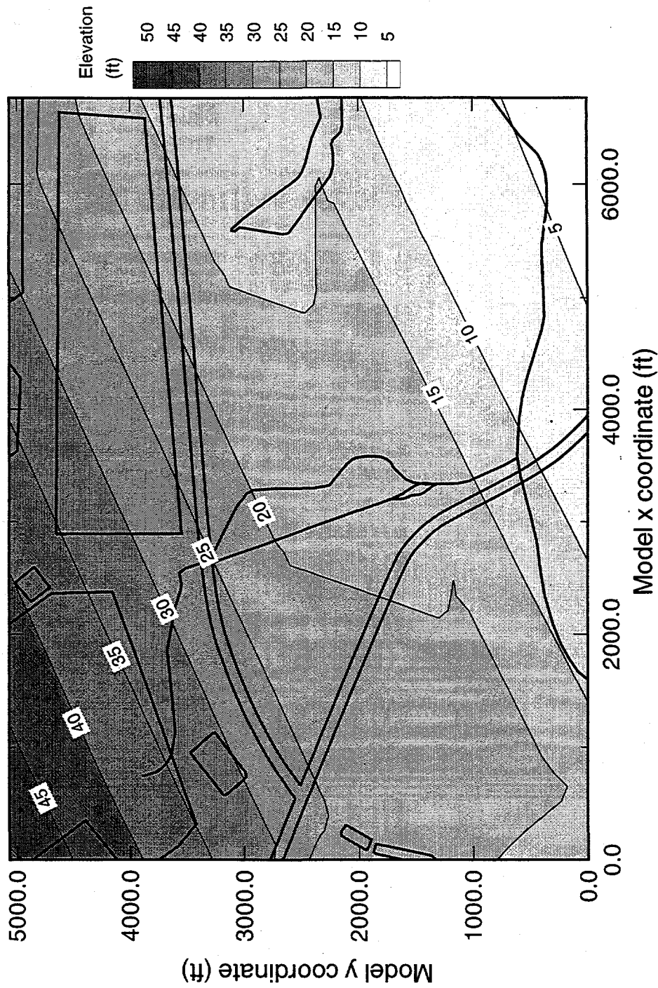
Figure 9. Structure contour map for the top of the Meyers Branch confining system (feet above mean sea level).
