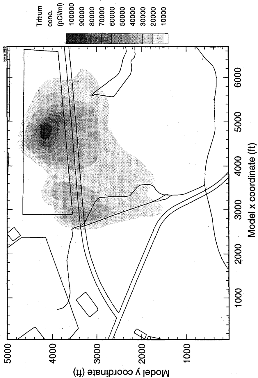
Figure 57f. Contour plot of predicted "lower" aquifer zone tritium concentration for 1985.
