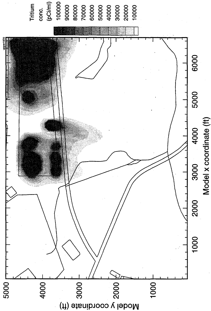
Figure 56c. Contour plot of predicted "upper" aquifer zone tritium concentration for 1970.
