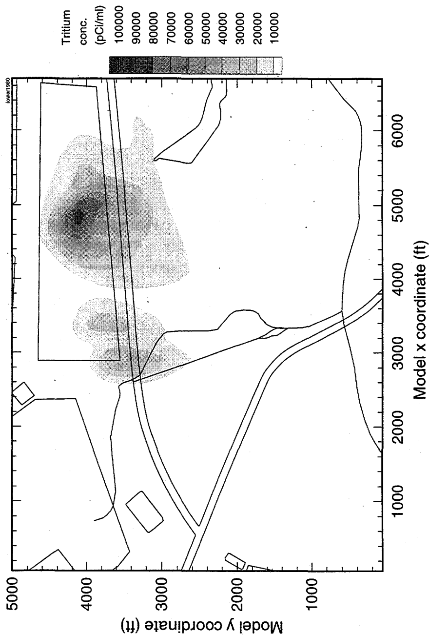
Figure 57e. Contour plot of predicted "lower" aquifer zone tritium concentration for 1980.
