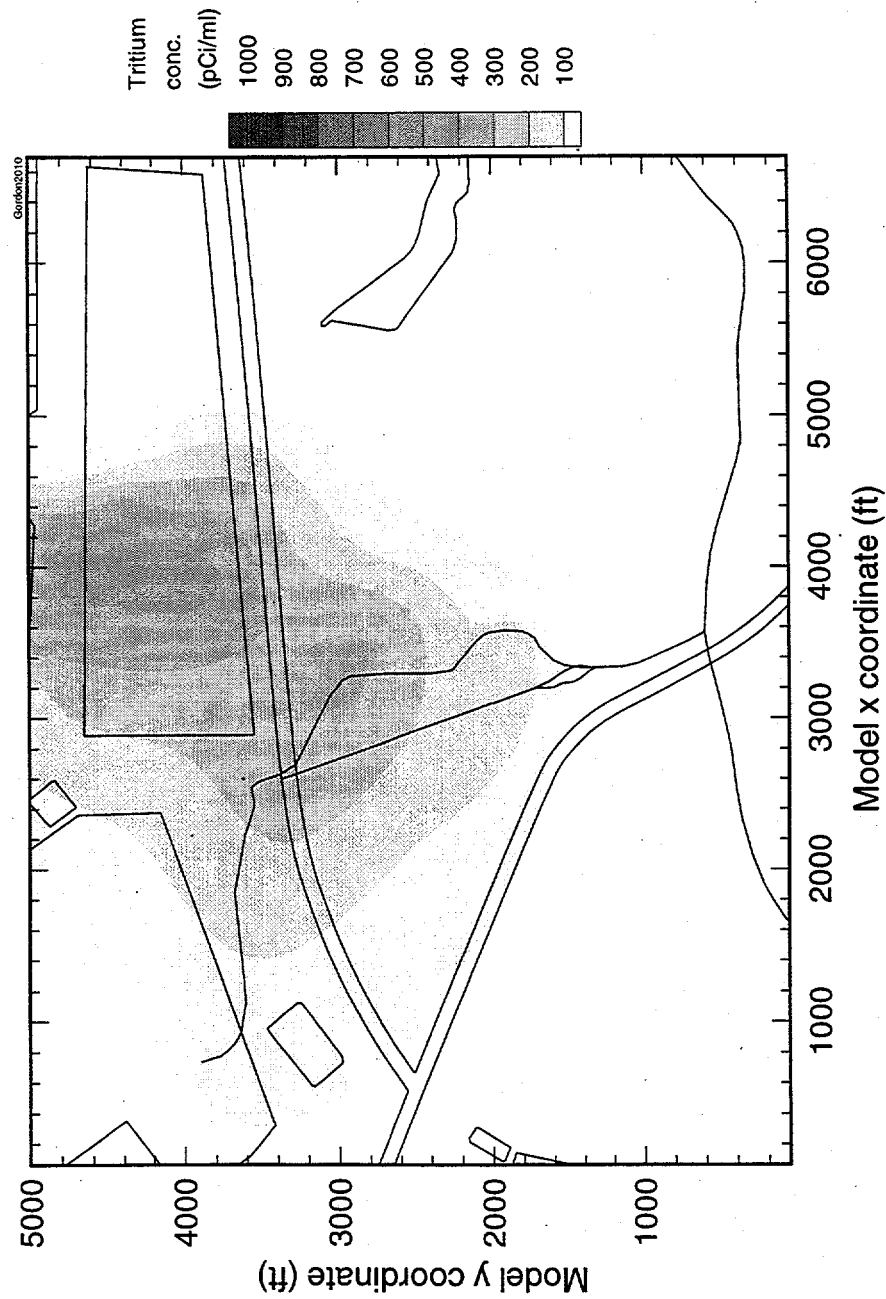
Figure 58k. Contour plot of predicted Gordon aquifer tritium concentration for 2010.
