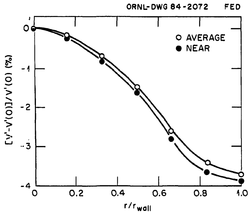
Fig. 8. Comparison of V' profile for helical axis ATF, between 3-D and average method calculations. Parameters are the same as in Fig. 4.
