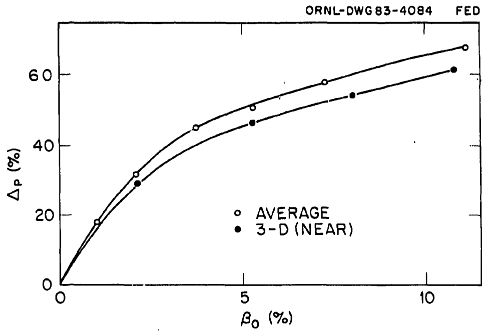
Fig. 5. Shift, (\Delta p) as a function of \beta_0 for the helical axis ATF.
