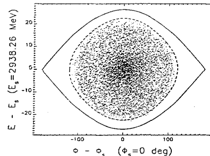
Figure 2: Rf bucket and bunch phase-space distribution from RCS-I at injection into RCS-II. The dotted line indicates the contour enclosing an area of 3.7 eV s.
