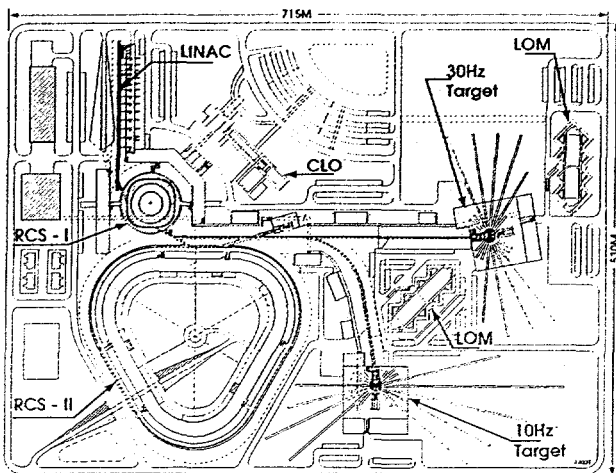
Figure 1: Site-independent 5-MW facility layout.
