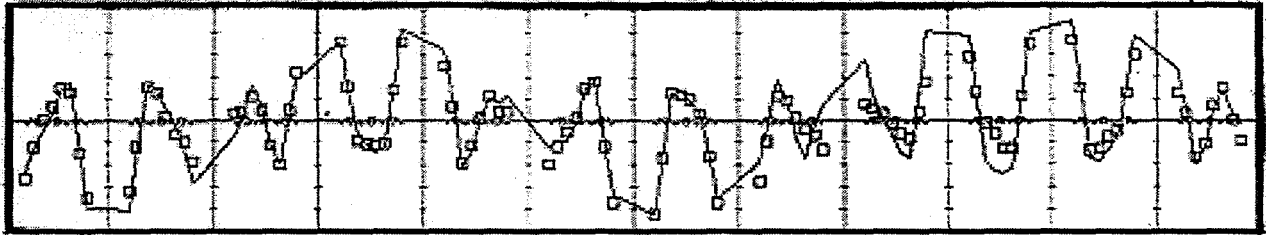
Figure 2. Horizontal closed-orbit distortion around the entire storage ring ( \pm 200\mu full scale) as measured on 9/12/96 (open symbols) and simulated by TRACY V (continuous line), assuming a progressive girder deformation of up to 31\mu .
