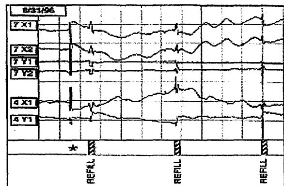
Fig. 3. Horizontal (X) and vertical (Y) ID-BPM signals from sectors 4 and 7, taken on 8/31/96. Grating units correspond to 150\mu , vertically, and 1 hour, horizontally. The illustration shows 1-hour oscillations, long-term drift, and a 10-min. step change (marked by an asterisk at the bottom). Signals have no validity during refill times.
