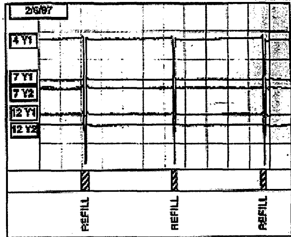
Figure 5. Vertical ID-BPM signals observed on 2/6/97 after substantially improving the temperature-stabilization. Grating units 150 \mu , vertically, and 1 hour, horizontally.
