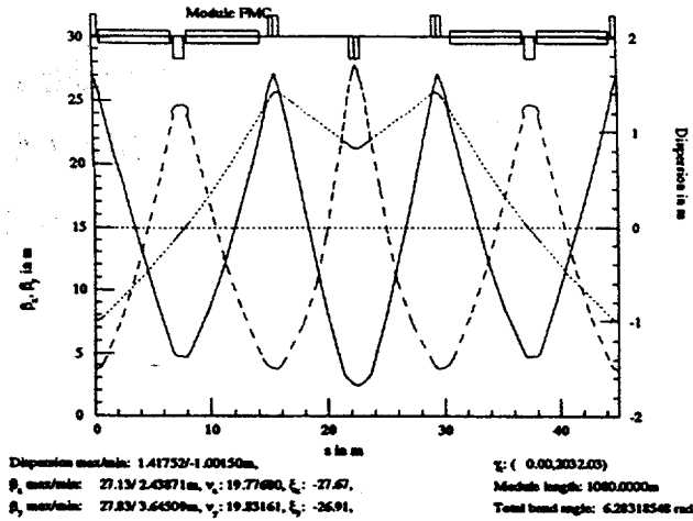
Figure 2: Imaginary \gamma_t lattice with missing dipole FODO cells.
