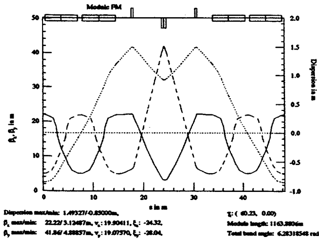
Figure 3: The missing dipole FODO cell lattice with combined function dipoles.
