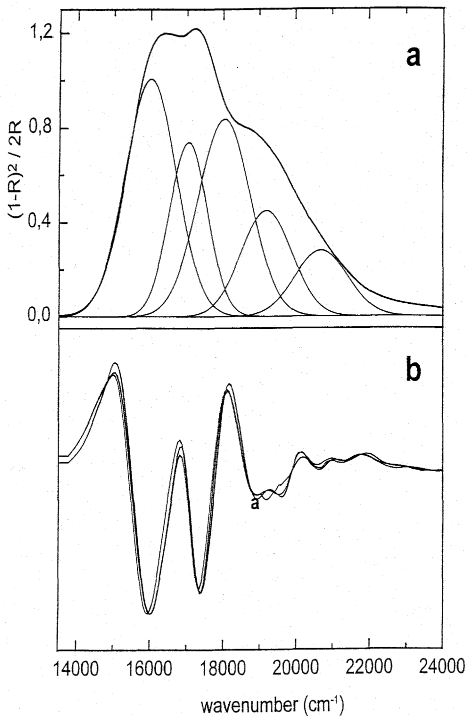
FIGURE 3. (a) The visible spectrum of the 7.9 wt% Co(II) erionite sample dehydrated at 350^{\circ}\text{C} , with deconvolution of the spectrum into Gaussian bands, and (b) the second derivative mode analysis of the visible spectra of Co(II) erionite containing 3.2, 7.9, and 8.2 wt% Co(II).
