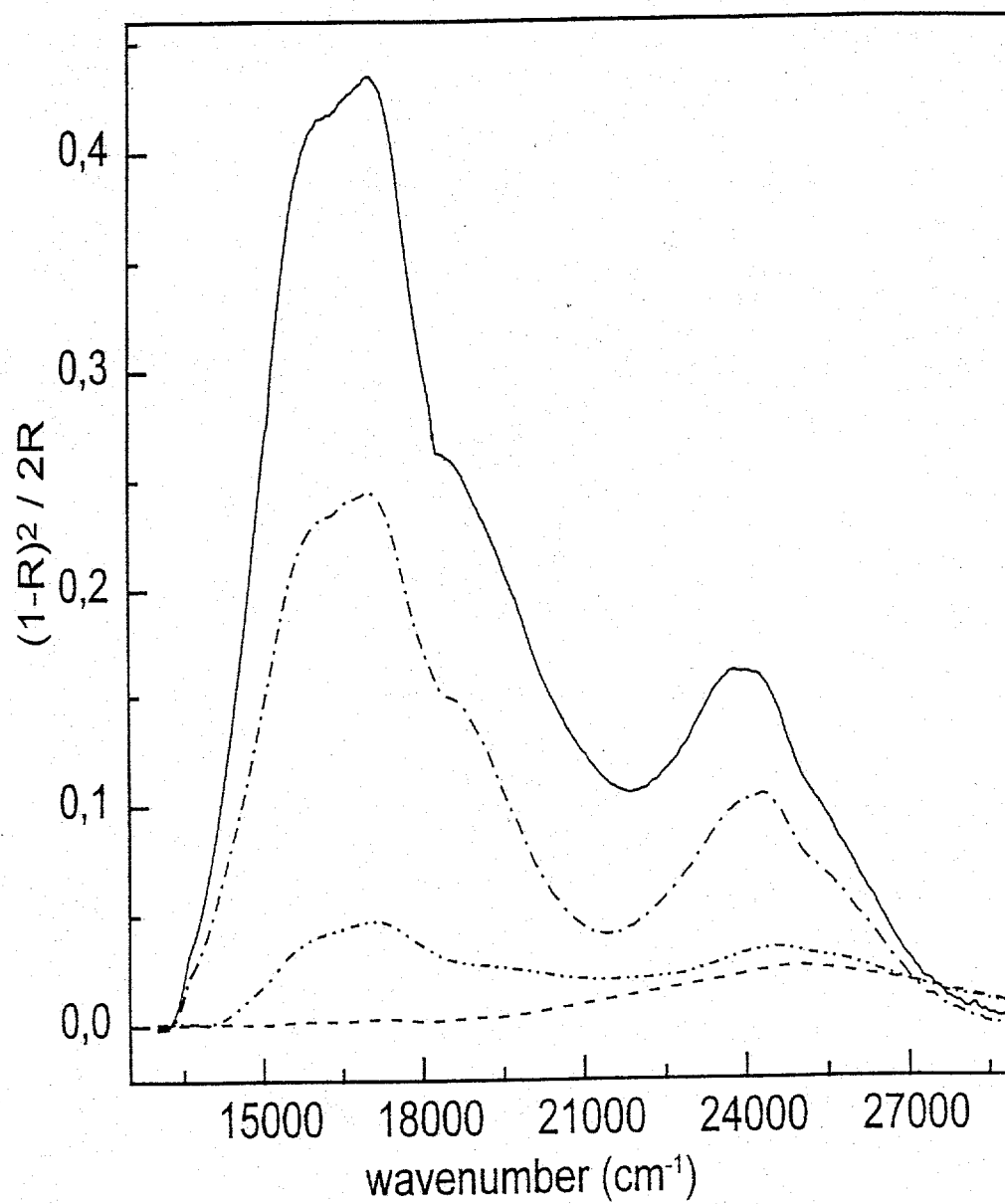
FIGURE 8. The effect of the Co(II) concentration on the Vis spectrum of 0.3, 1.5, 3.2, and 8.2 wt% Co(II) erionite samples dehydrated at 525^\circ\text{C}
