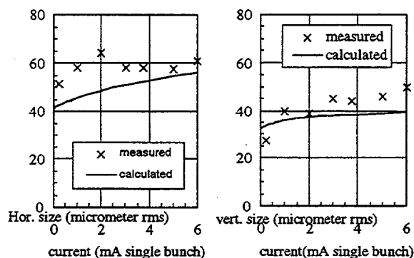
Figure 2. Measured and calculated beam sizes in the ALS for beam energy of 1522 MeV. Coupling was assumed to be 1.5 %.
