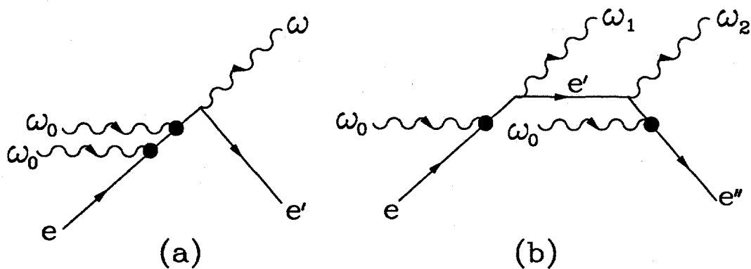
Fig. 2. Diagrams representing (a) n = 2 nonlinear Compton scattering, and (b) double ordinary Compton scattering.
