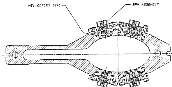
Figure 8B. PEP-II LER arc position monitor
