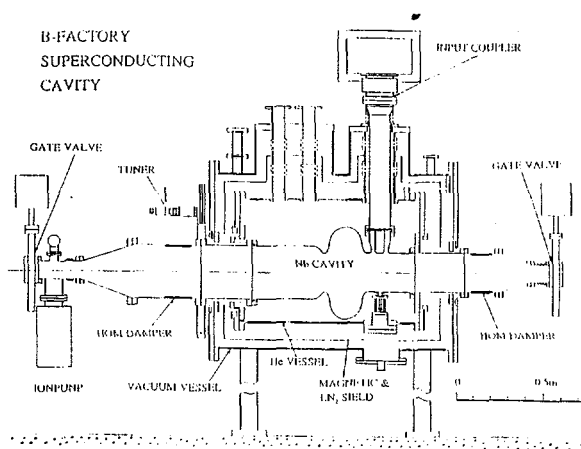
Figure 2B. KEKB superconducting cavity
