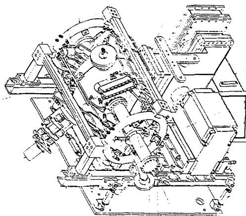
Figure 2C. PEP-II copper RF Cavity
