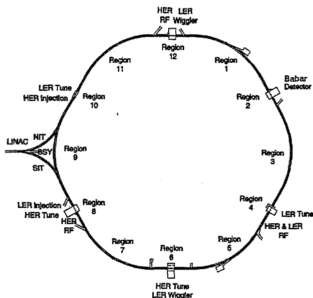
Figure 1B PEP-II B Factory Overview
