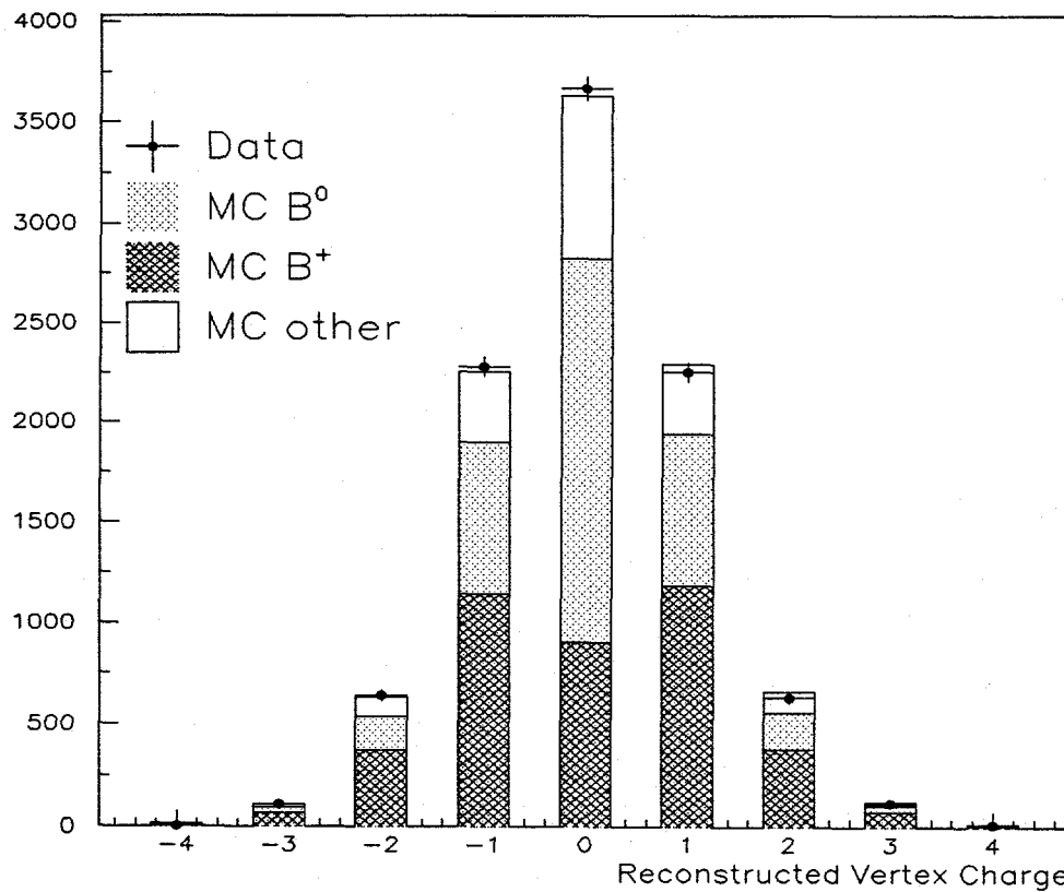
Figure 2: Reconstructed vertex charge for Monte Carlo (histogram) and data (points).
