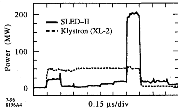
Figure 4. High-power test of the SLED-II prototype.
