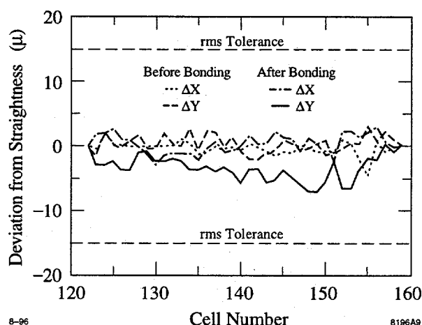
Figure 9. Alignment after diffusion bonding of a short stack of cells in the Damped-Detuned structure.
