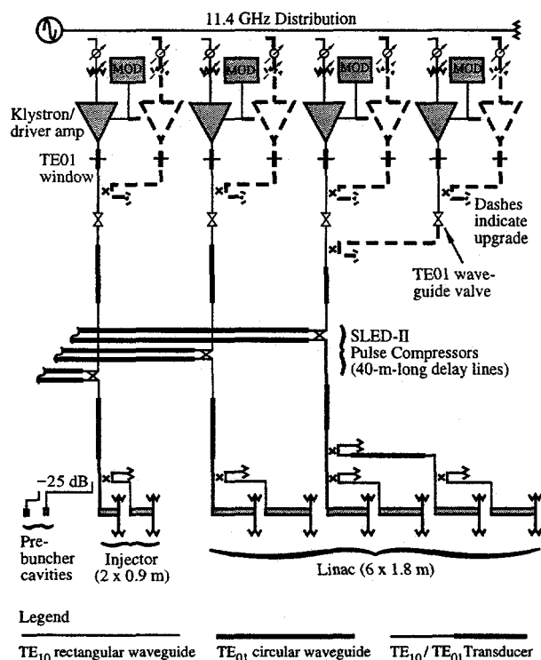
Figure 1. A schematic of the NLCTA rf system
