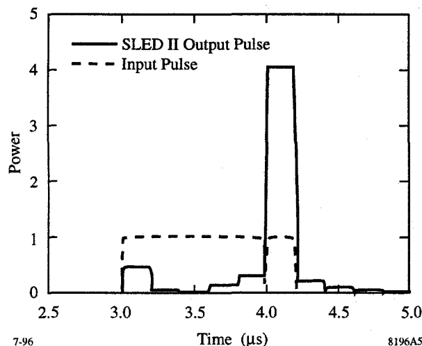
Figure 5. Low-power test of Injector SLED-II system.
