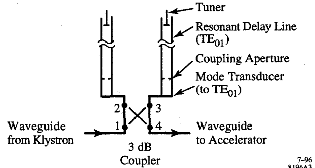
Figure 3. A schematic of the SLED-II rf compression.
