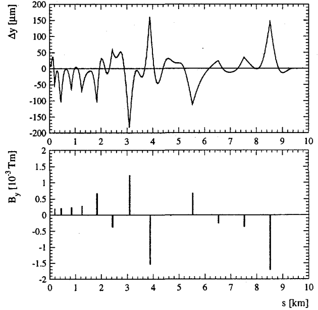
Figure 1: Example of the beam-based alignment algorithm with perfect BPM's and RF-BPM's. The initial random quadrupole misalignment was 100\ \mu\text{m} rms. The alignment is done in 14 sections and 15 iterations. At the end of each section a dipole corrector is used to launch the beam into the next section. The upper plot shows the misalignment \Delta y of quadrupoles, RF-structures and BPM's after alignment. The lower plot shows the integrated fields of the dipole correctors.
