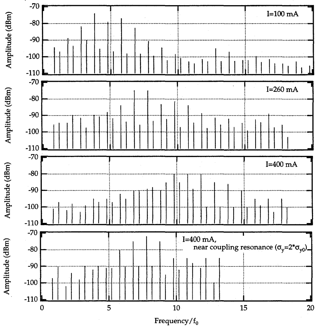
FIGURE 2. Amplitudes of residual vertical betatron sidebands measured in the 320/328 fill pattern at 3 total beam currents.
