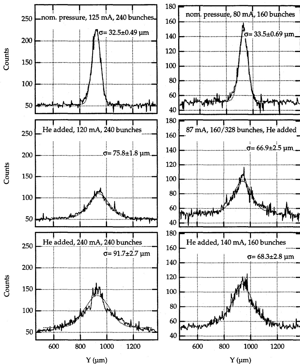
FIGURE 5. Vertical profile through the bunch center for nominal pressures and with helium added. The left column shows the case for 240/328 bunches and the right column is for 160/328 bunches. Each profile is fitted to a gaussian with the RMS shown.
