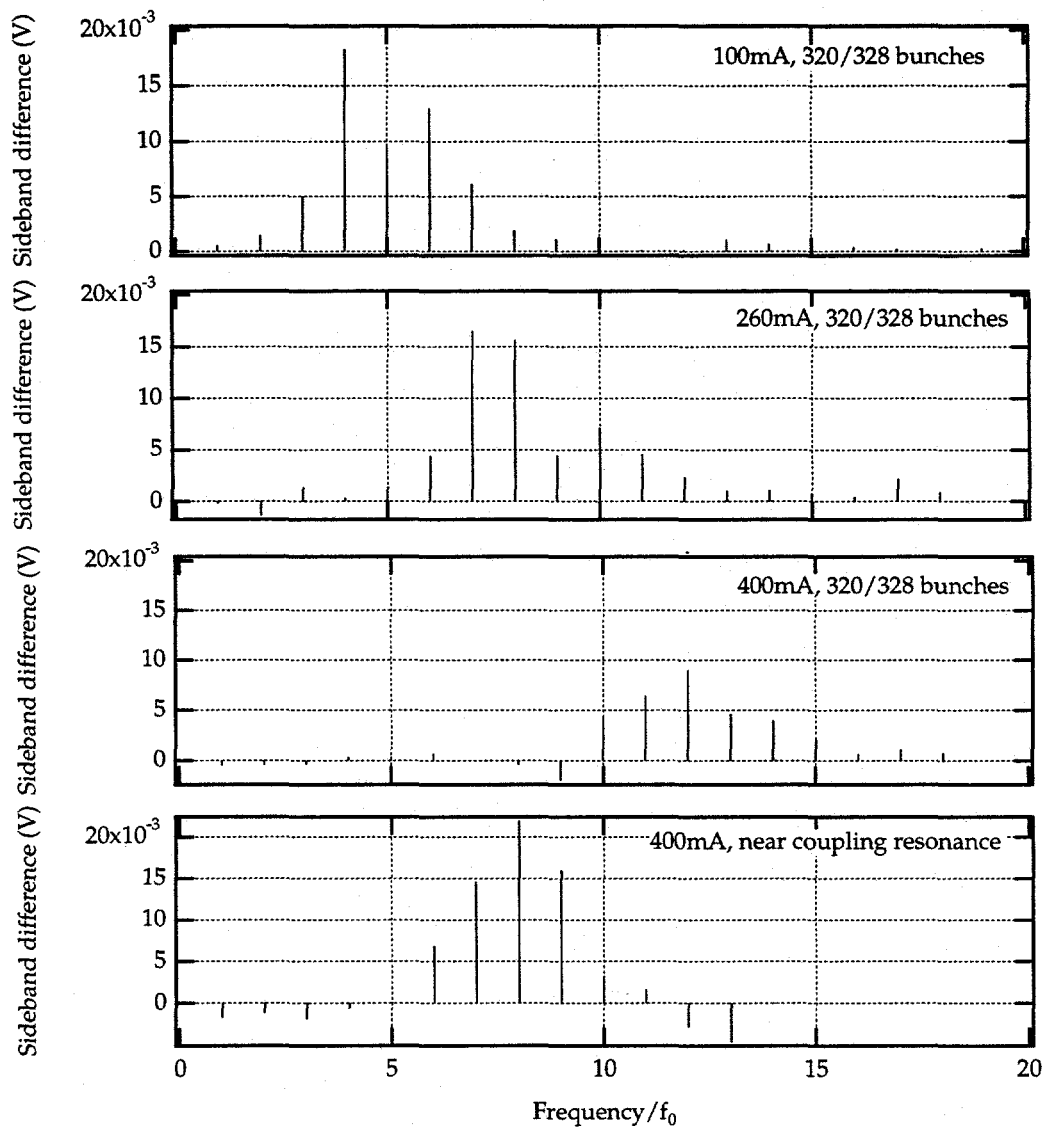
FIGURE 3. Difference between lower and upper residual vertical betatron sidebands measured in the 320/328 fill pattern at 3 total beam currents.
