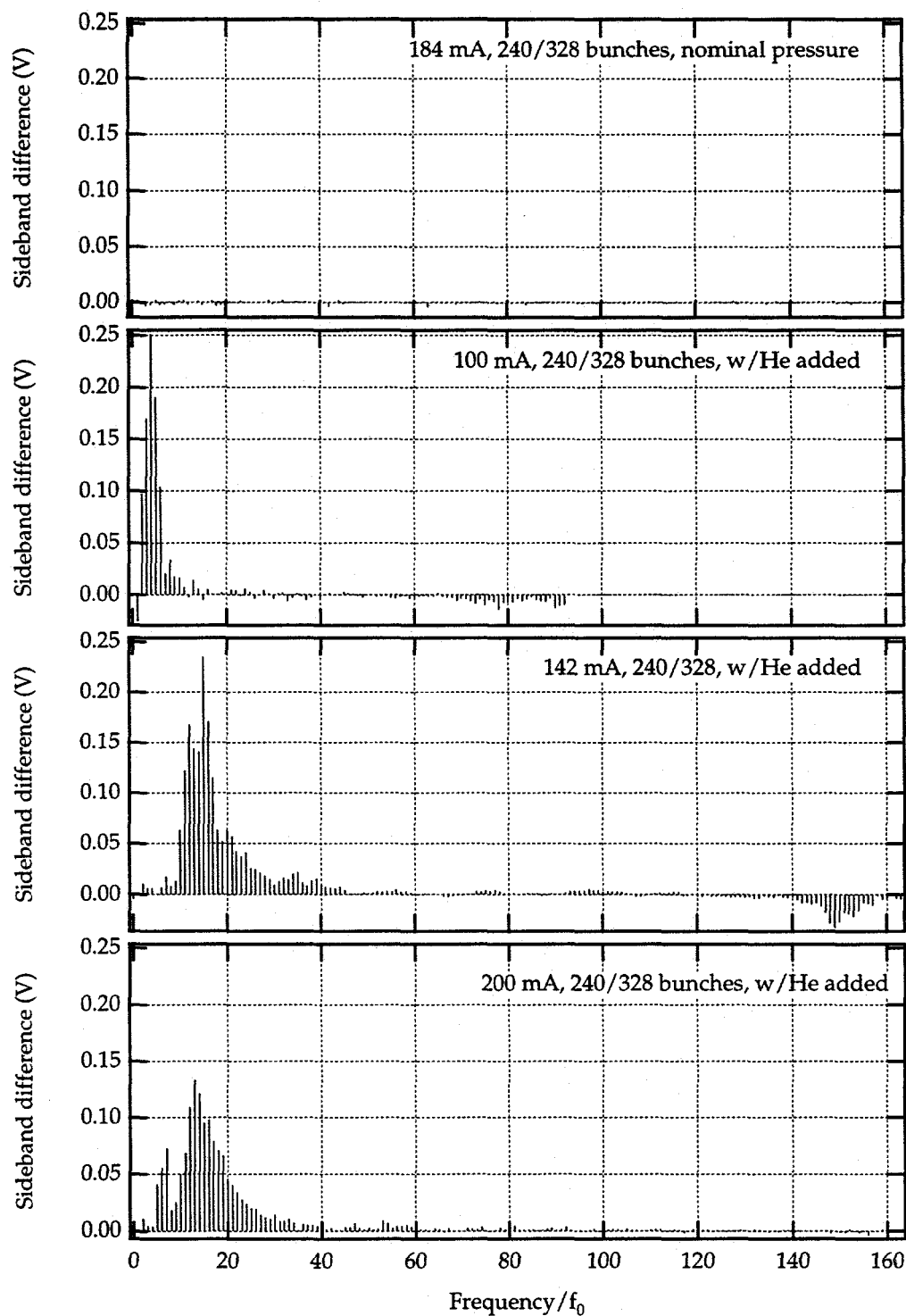
FIGURE 6. Difference between lower and upper residual vertical betatron sidebands measured in the 240/328 fill pattern at for several different conditions. A coherent signal appears when helium is added to the vacuum.
