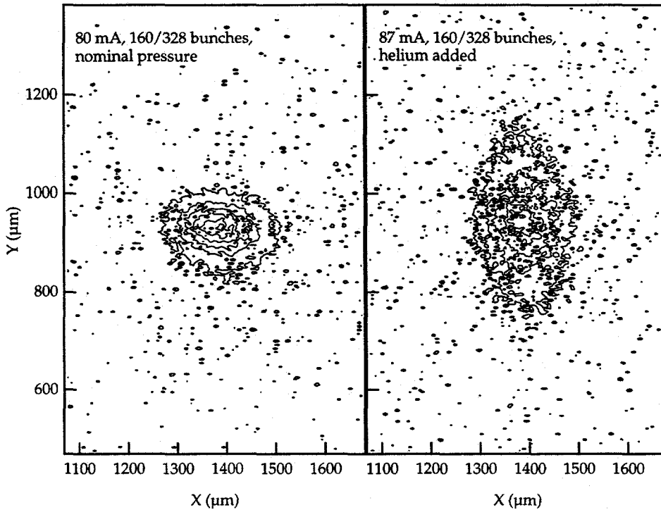
FIGURE 4. Transverse profile images (shown as contour plots) of the beam for nominal pressures and with helium added.
