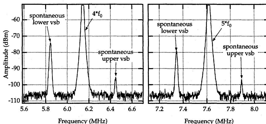
FIGURE 1. Raw spectrum of vertical pickup shown near the 4th and 5th revolution harmonics.
