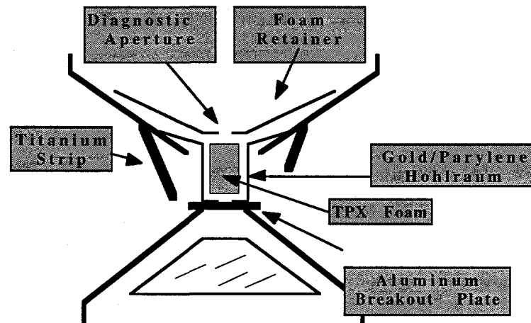
Fig. 2. Illustration of the target's major components.
