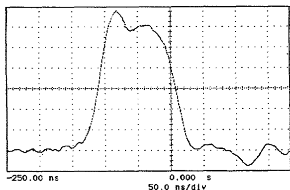
Figure 4: Load current.
