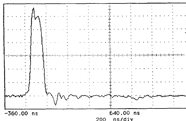
Figure 5: Load current with "after pulse" at 850 nsec.
