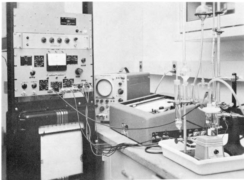
Figure 21. A.C.-D.C. polarograph, cell assembly, and related equipment.
