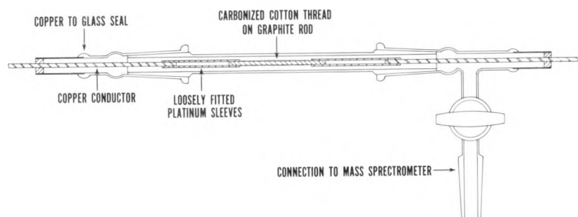
Figure 1. Device for conversion of oxygen to carbon dioxide.
