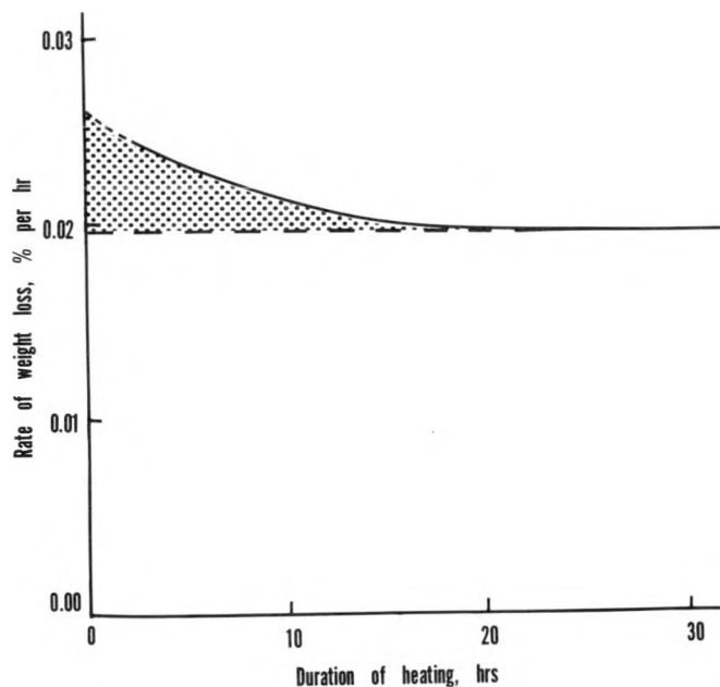
Figure 11. Stability of THAM during heating at 110°C.
