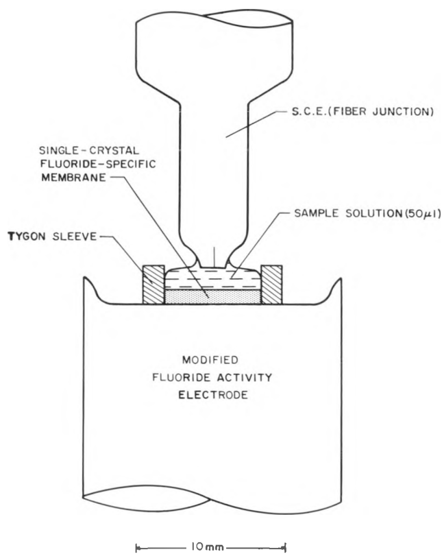
Figure 19. Fluoride electrode microcell and S.C.E.
