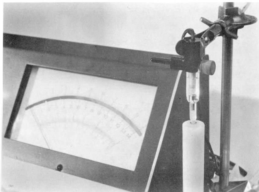
Figure 20. Fluoride electrode microcell assembly.
