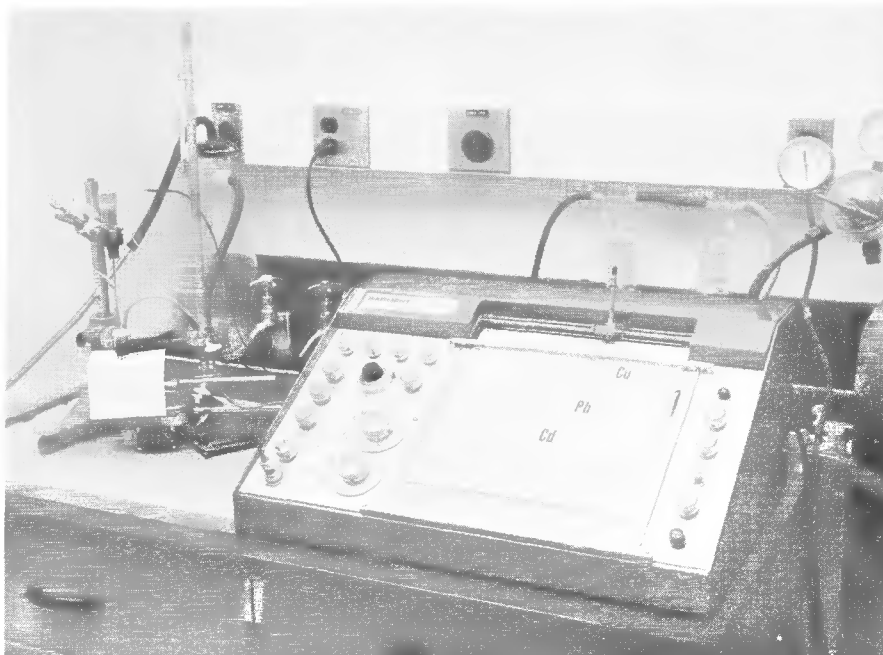
Figure 10. Apparatus for anodic stripping polarography.
