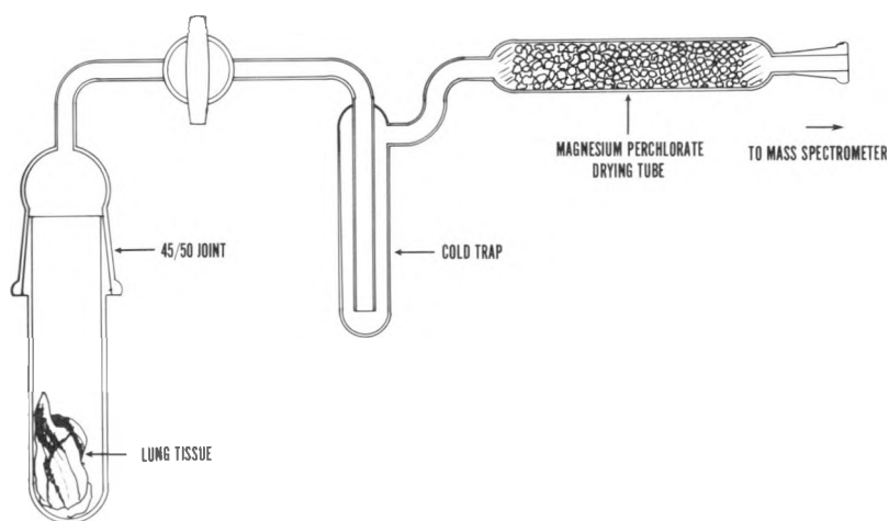
Figure 8. Apparatus for evaluation and collection of gases evolved from lung tissue.
