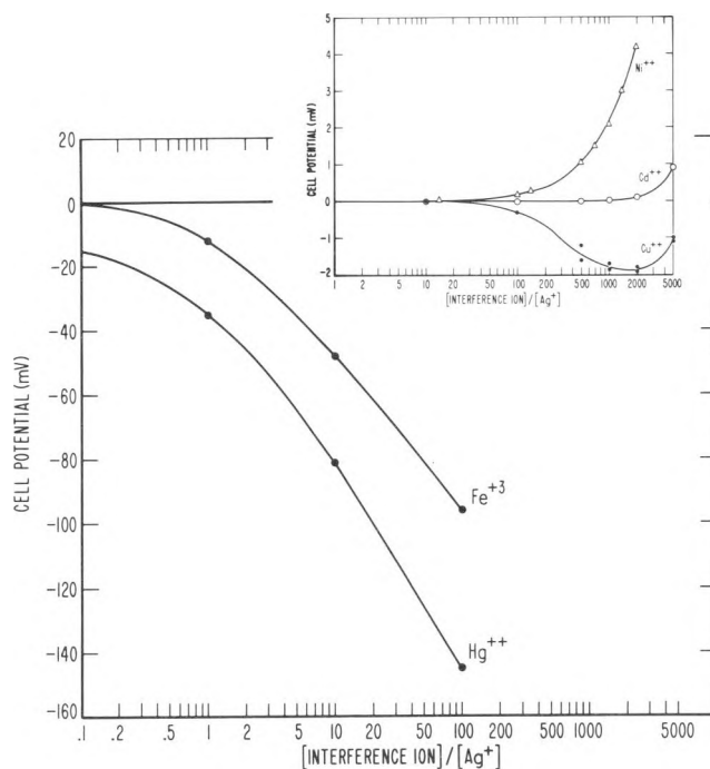
Figure 18. Cation interference curves at [\text{Ag}^+] = 10^{-4} \text{ M} .
