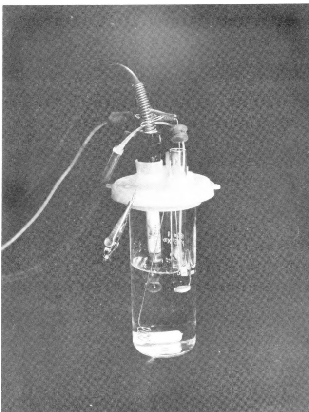
Figure 12. Coulometric cell for microtitrations of halides.
