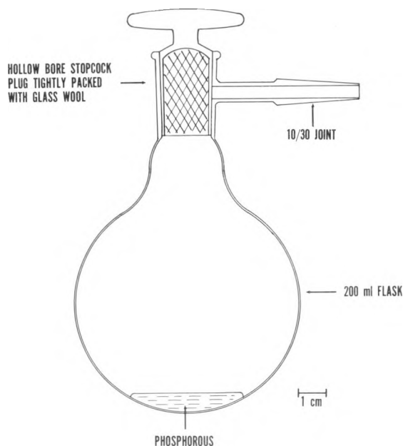
Figure 2. Flask for oxygen determination.
