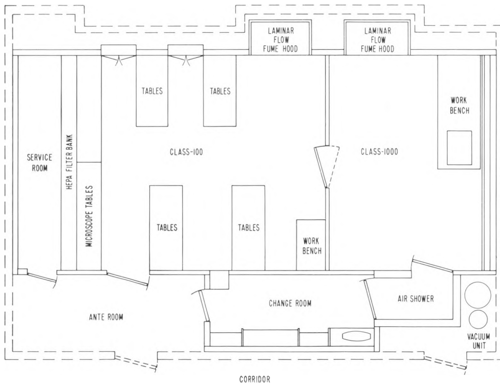
Figure 24. General layout for clean room facility.
