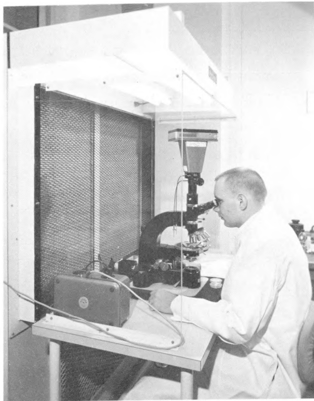
Figure 22. Laminar flow clean bench.
