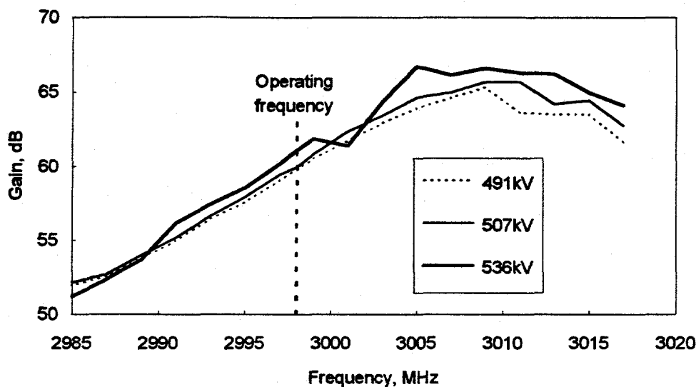
FIGURE 2. Small signal gain of the 150-MW klystron verses frequency.
