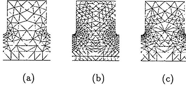
Figure 2. (a) Initial mesh ; (b) Uniform refinement ; (c) Adaptive refinement .
