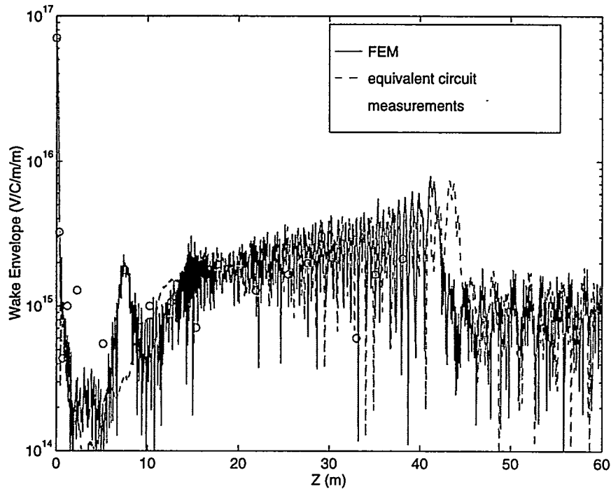
Figure 4. Wake envelopes obtained from FEM and equivalent circuit calculations.
