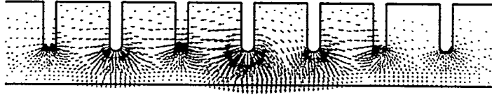
Figure 3. Electric field pattern (from cell 163 to 170) of mode 166 .
