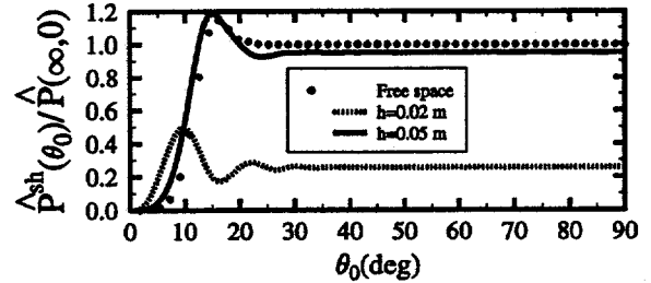
Figure 2: Transient power loss of a bunch, due to curvature-induced self-interaction in the presence of parallel plates, with \rho = 1 m, \sigma_s = 1 mm, and various plate spacings h . Here \theta_0 is the angle of bunch center into the bend.
