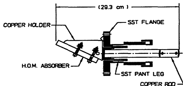
FIGURE 2. FEL HOM load and heat sink design.
