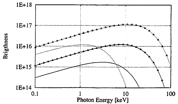
Figure 3: Brightness [ \frac{\text{photons}}{(\text{s} \cdot \text{mm}^2 \cdot \text{mrad}^2 \cdot 0.1\% \text{b.w.})} ] from lattice bend magnets and high-field bend magnets (triangles) at the present ALS (solid lines) and the ALS-N (dashed lines).
