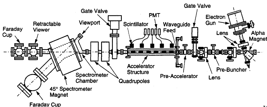
Figure 1: Layout of Accelerator Structure Test Area.
