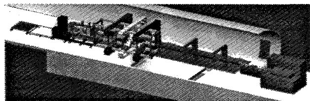
Conceptual layout of the LEDA accelerator, showing injector, RFQ (behind waveguides), a section of the CCDTL, and the shielded beam stop.
