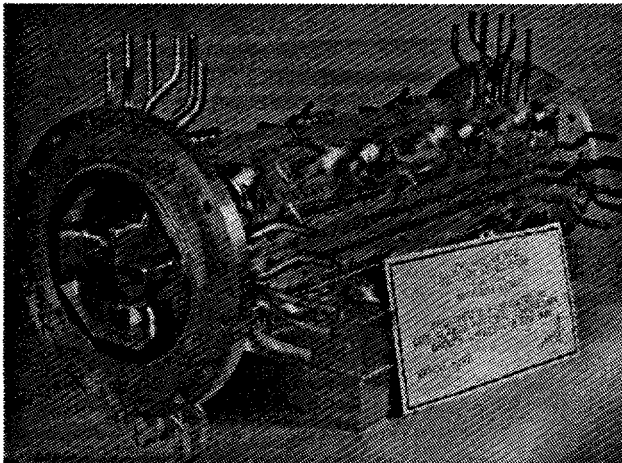
Photo of the first completed 1-m long section of the LEDA RFQ.
