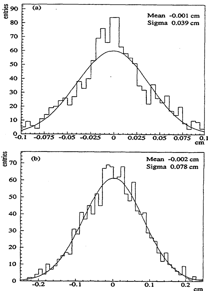
Fig. 6 Particle hit residuals in the (a) azimuthal and (b) drift direction.
