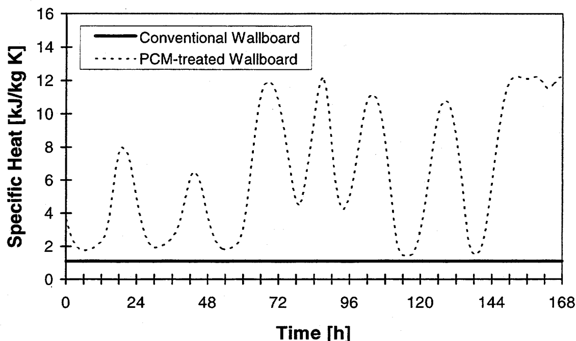
Figure 10: Specific Heat Capacity Variation for the Wallboard of the West Wall with Ventilative Cooling
