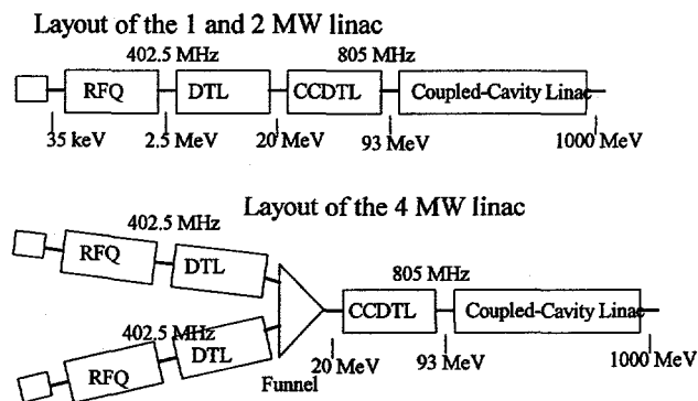
Figure 1. Layout of the accelerator structures for the 1, 2, and 4 MW NSNS linacs.
