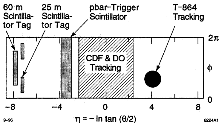
Figure 1: MiniMax lego acceptance.
