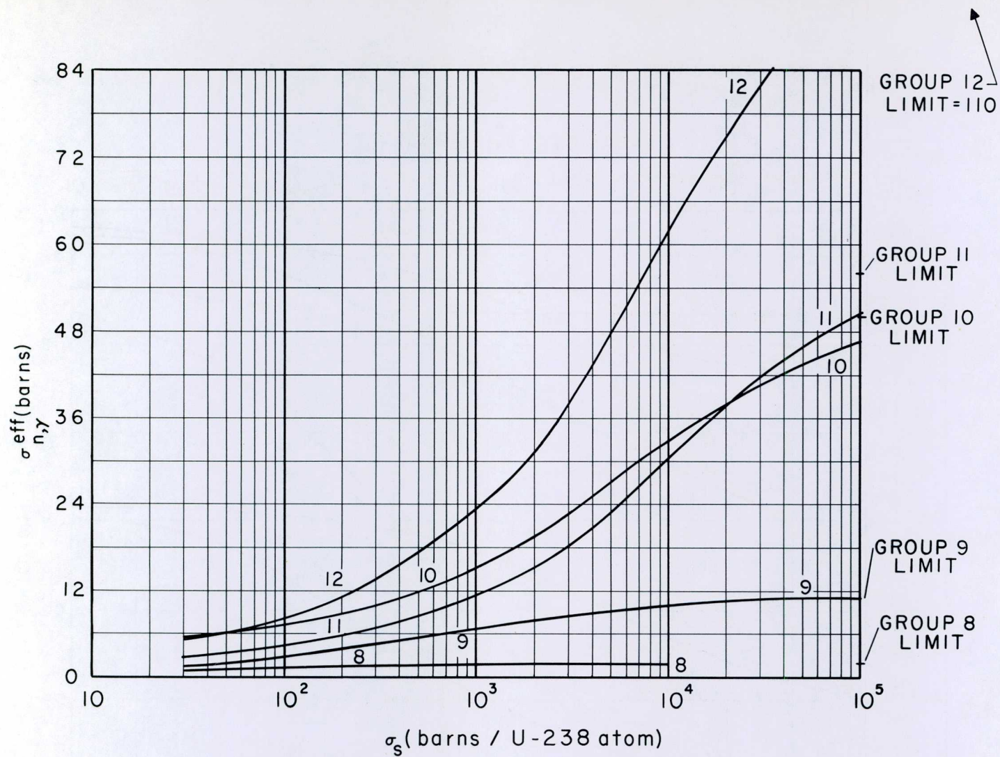
Fig. 16 Shielded Capture Cross Sections for U^{238} .
