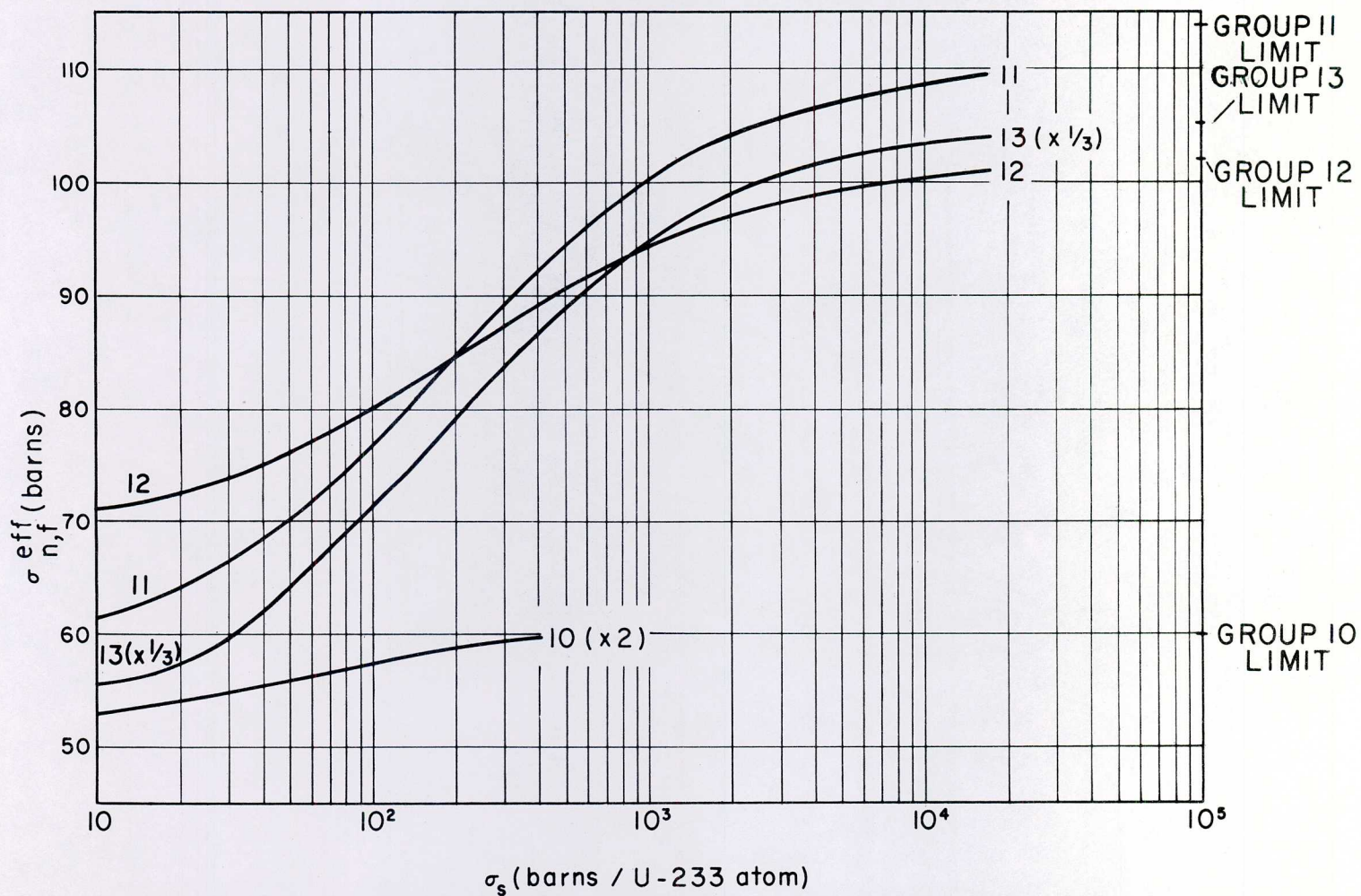
Fig. 13 Shielded fission cross sections for U^{233} .
