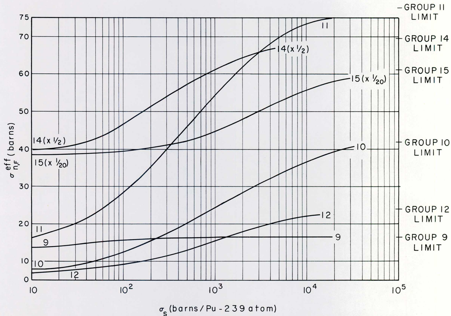
Fig. 15 Shielded Fission Cross Sections for \text{Pu}^{239} .
