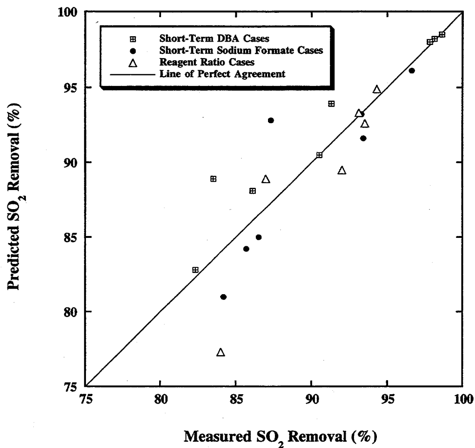
Figure 3-1. Comparison of Measured and FGDPRIISM Predicted SO 2 Removal
