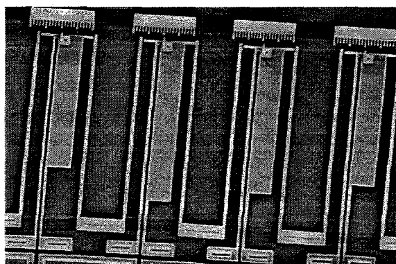
Figure 2. Four independent 150 \mu\text{m} long actuators, each instrumented with deflection scales and two test beams for measuring force in both forward and backward deflection.
