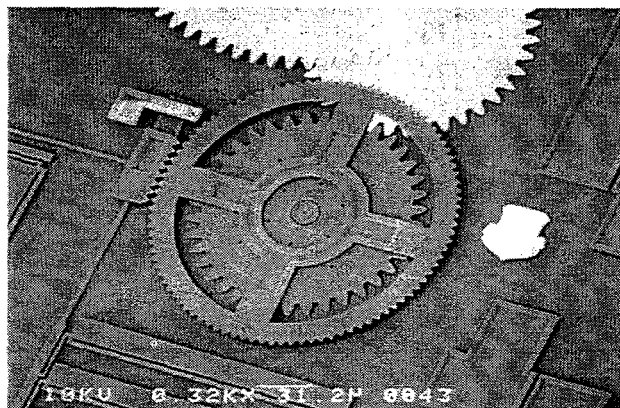
Figure 7. Rotary stepper motor. Main two-level gear adapts thermal actuator stroke to tooth pitch of standard, software-generated Sandia gears. Upper gear is planarized Poly-3.
