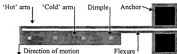
Figure 1. Schematic view of an electrothermal actuator.
