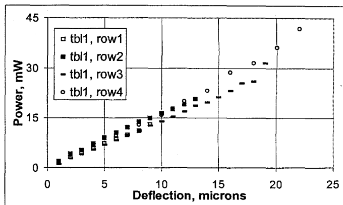
Figure 3. Deflection versus power for the actuators listed in Table 1. Maximum voltages applied to the 150 , 200 , 250 , and 300 \mu\text{m} long actuators were 8.3 , 9 , 13 , and 13.7 \text{ V} respectively.
