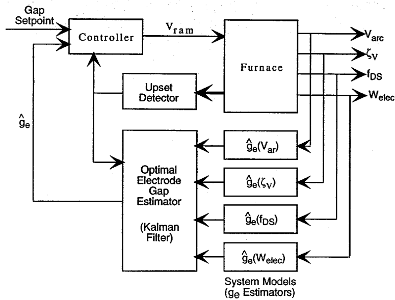
Figure 2. A block diagram of a multiple input, electrode gap controller as described in the text.
