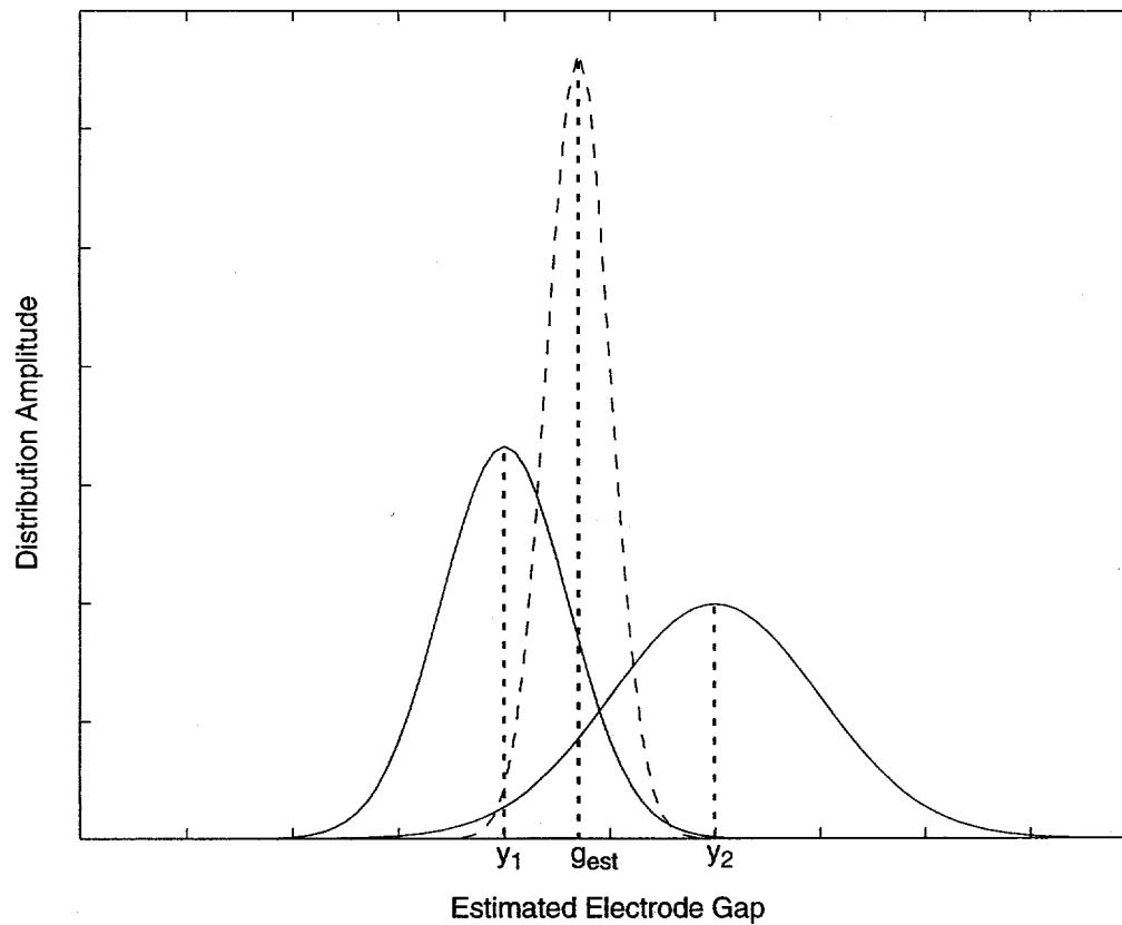
Figure 3. Example of combining two independent gap estimates to obtain an optimal estimate of statistically greater certainty.
