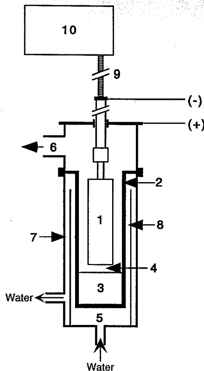
Figure 1. A simplified schematic of a VAR furnace. Key: 1) electrode; 2) copper crucible; 3) ingot; 4) electrode gap; 5) cooling water; 6) vacuum port; 7) furnace body; 8) cooling water guide; 9) ram drive screw; 10) ram drive motor assembly.
