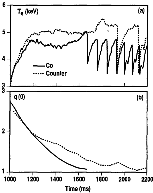
FIGURE 4. Time histories of (a) central electron temperature and (b) central safety factor for matched co and counter FWCD discharges ( B_T = 1.9 T, \bar{n} = 1.3 \times 10^{19} \text{ m}^{-3} , P_{\text{nb}} = 2.6 MW, P_{\text{fw}} = 2.1 MW).
