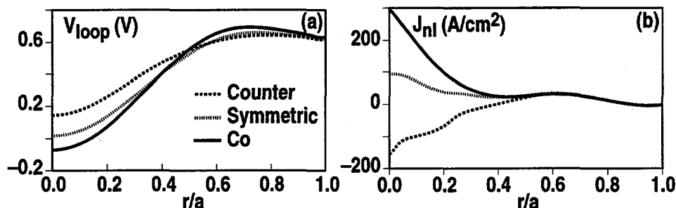
FIGURE 1. Radial profiles of (a) loop voltage and (b) non-inductive current density for three antenna phasings ( B_T = 2.1 T, \bar{n} = 1.9 \times 10^{19} m -3 , P_{nbi} = 3.7 MW, P_{fw} = 2.2 MW).
