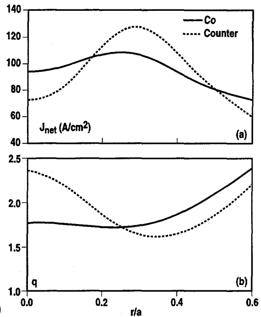
FIGURE 5. Radial profiles of (a) net current density and (b) safety factor at identical times for matched co and counter FWCD discharges ( B_T = 1.9 T, \bar{n} = 1.3 \times 10^{19} \text{ m}^{-3} , \bar{n} = 1.8 \times 10^{19} \text{ m}^{-3} , P_{\text{nb}} = 3.7 MW, P_{\text{fw}} = 2.2 MW).
