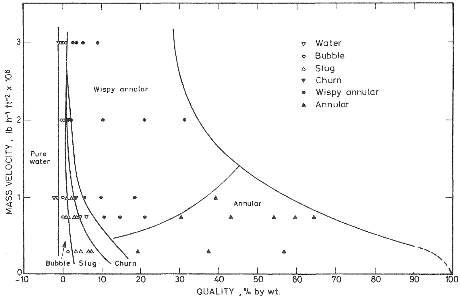
FLOW PATTERN DIAGRAM OBTAINED BY BENNETT ET AL (5) FOR STEAM-WATER FLOW IN A 0.5 INCH BORE TUBE AT 1000 lb/in 2 .
