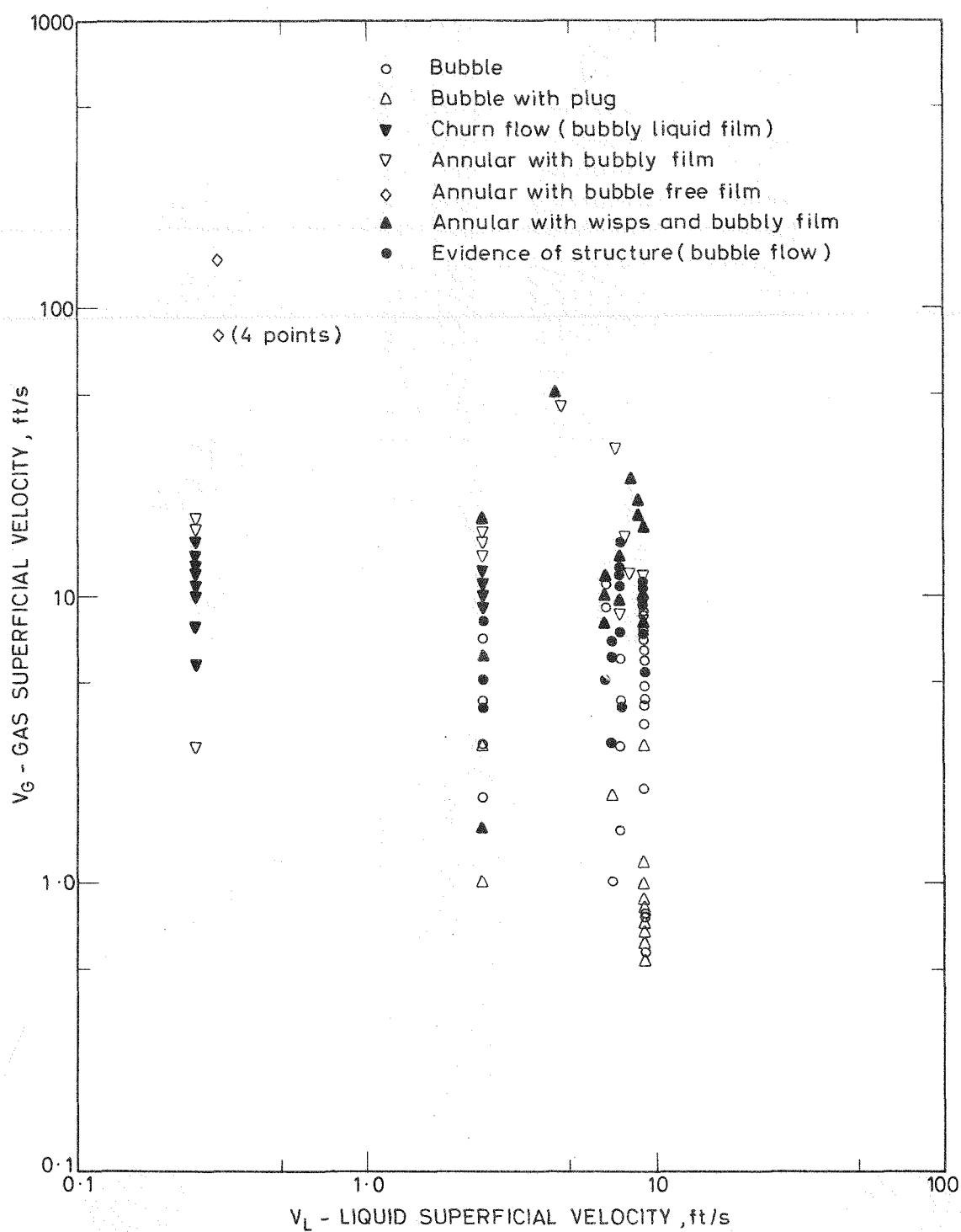
FLOW PATTERN MAP PLOTTED IN TERMS OF SUPERFICIAL VELOCITIES.
