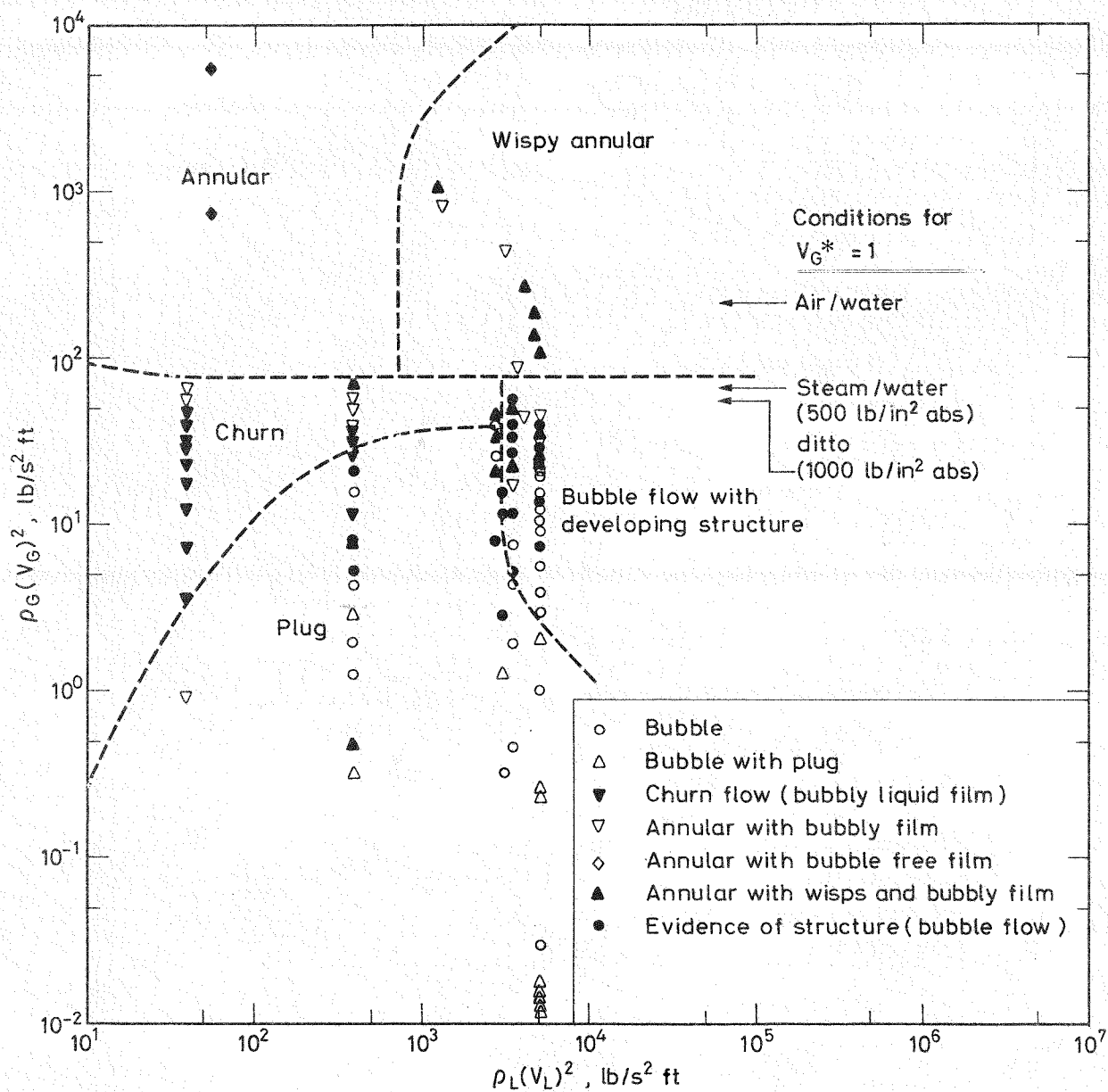
FLOW PATTERN MAP PLOTTED FROM DATA IN TABLE 1.
