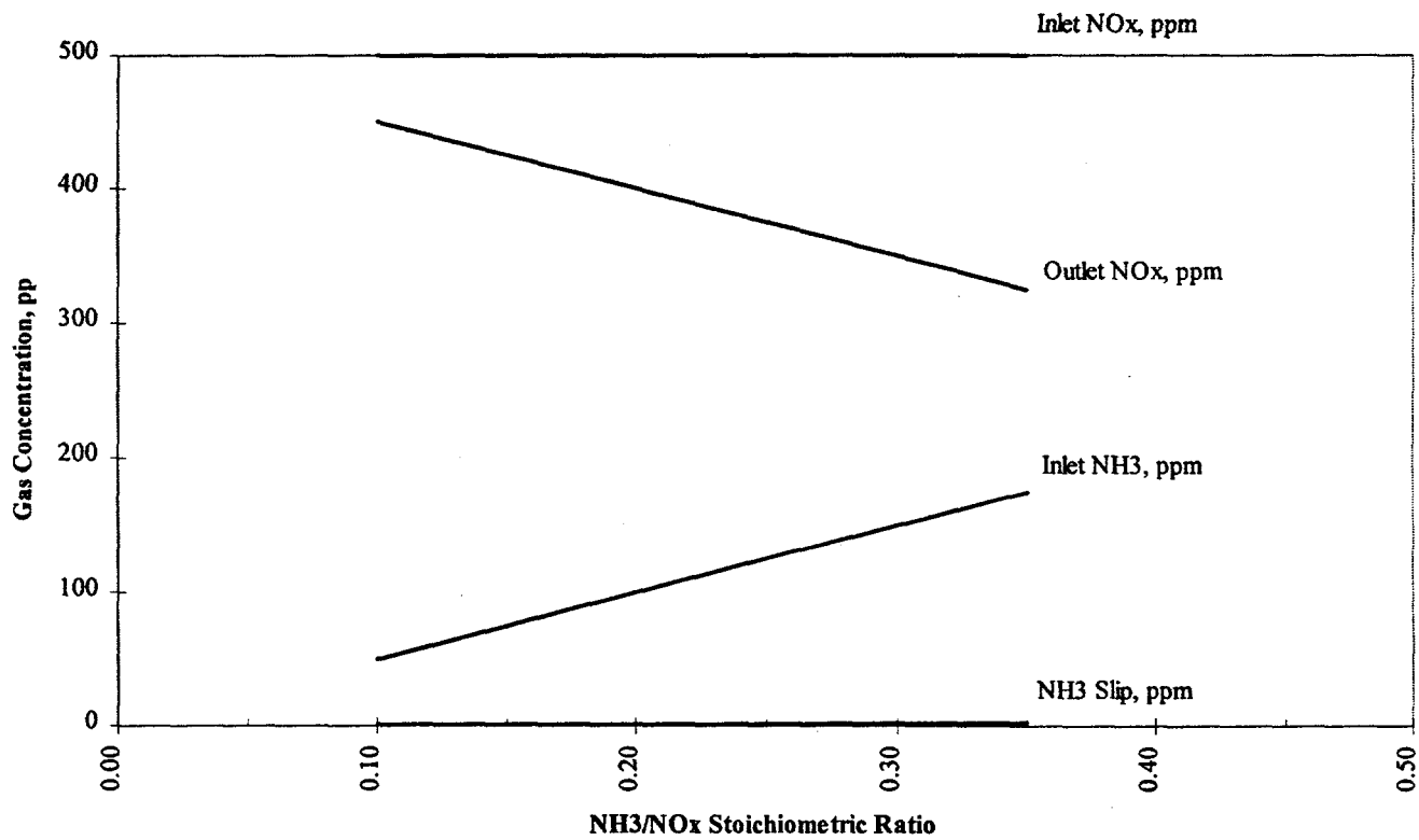
Figure 6 - \text{NO}_x Reduction
