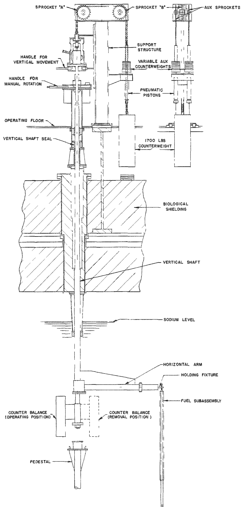
Figure 1. Modified Transfer Arm Mechanism
