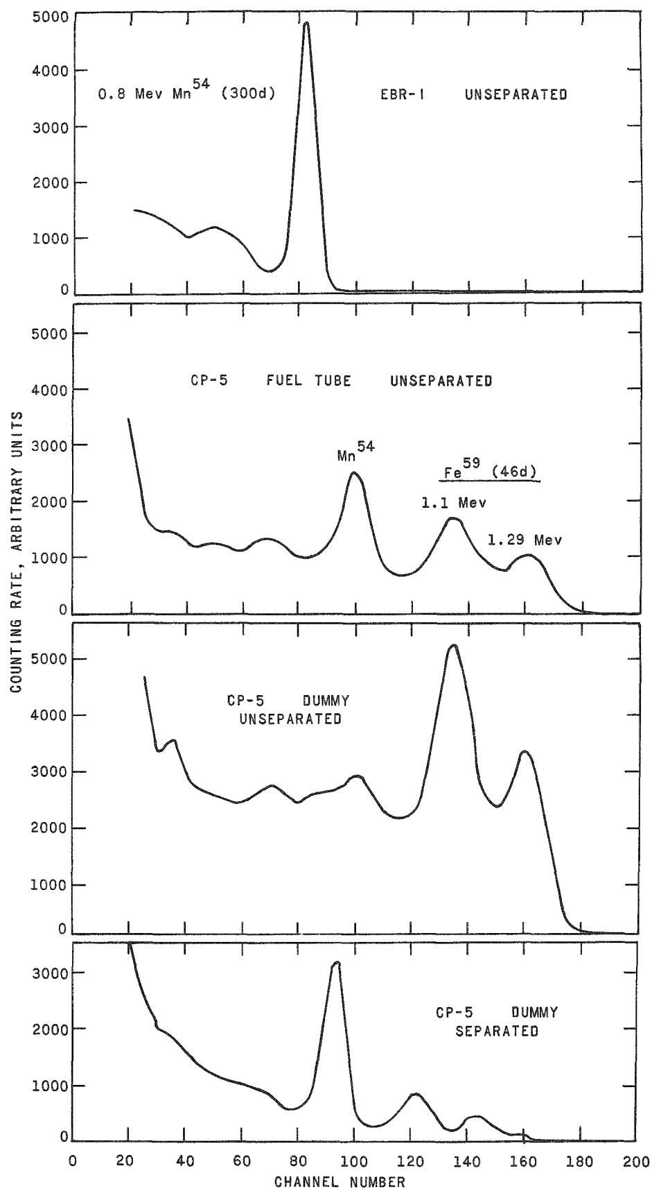
Figure 5. Typical Gamma-Ray Spectra from Irradiated Steel
