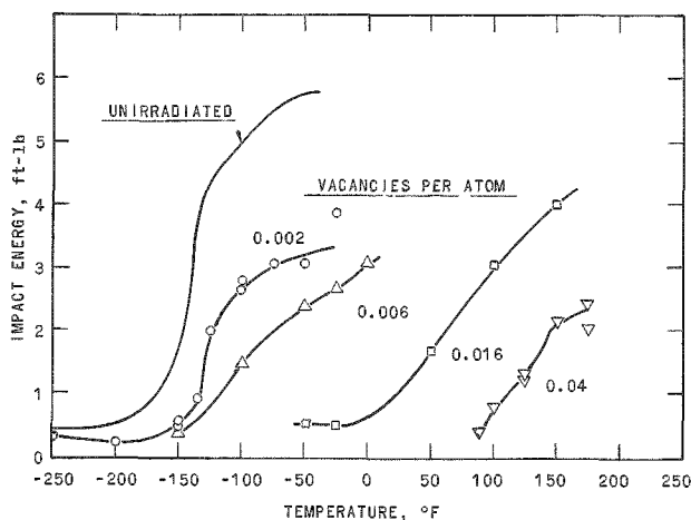
Figure 2. Impact Properties of SA-212B; EBR-I Irradiations
