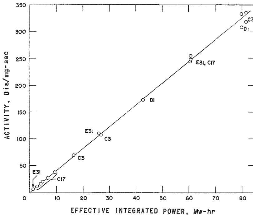
Figure 4. Correlation of \text{Mn}^{54} Activity with Predictions
