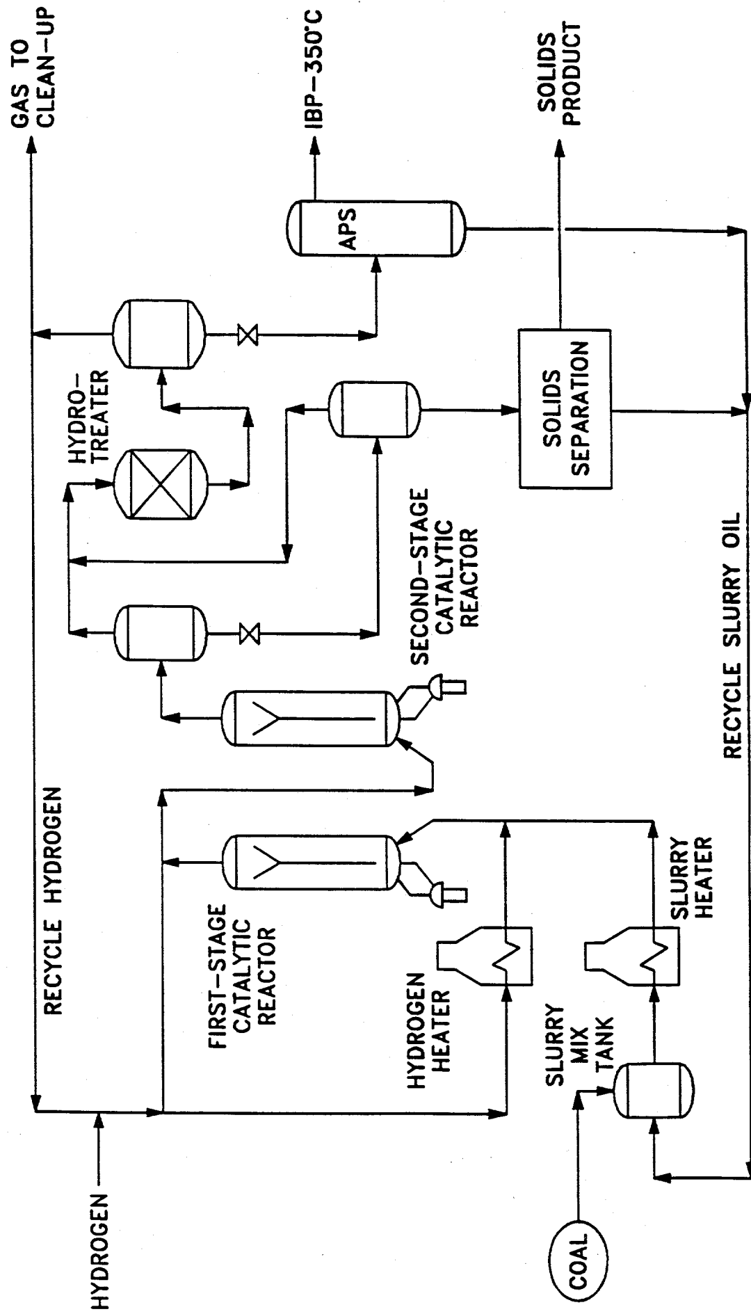
FIGURE 1.1 Simplified Flow Diagram of Catalytic Two-Stage Process
