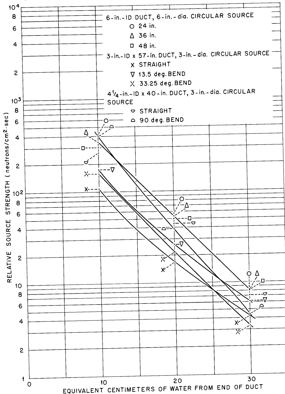
Fig. 27. Comparison of Relative Source Strengths ( n_0 ) from Various Ducts. Source area equal to duct mouth area.
