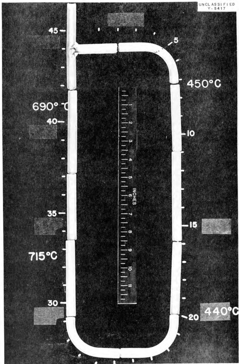
Fig. 40. Inconel Thermal Convection Loop Operated for 135 hr with Potassium Hydroxide Under a Hydrogen Atmosphere.
