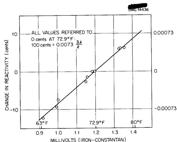
Fig. 19. Reactivity vs. Temperature.
