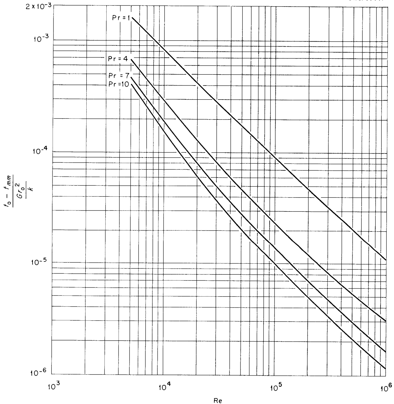
Fig. 48. Dimensionless, Wall-Mixed Mean Temperature Difference as a Function of Reynold's and Prandtl's Moduli for a Heat Transfer System with Insulated Pipe Walls.
