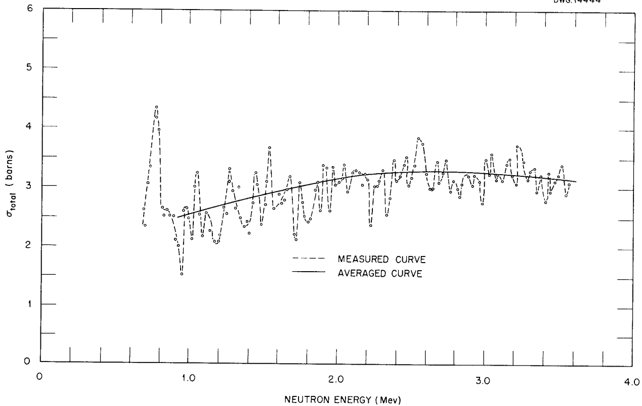
Fig. 31. Total Cross Section of Iron.
