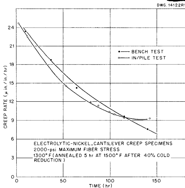
Fig. 50. Comparison of Bench and Inpile Creep Rates of Nickel.
