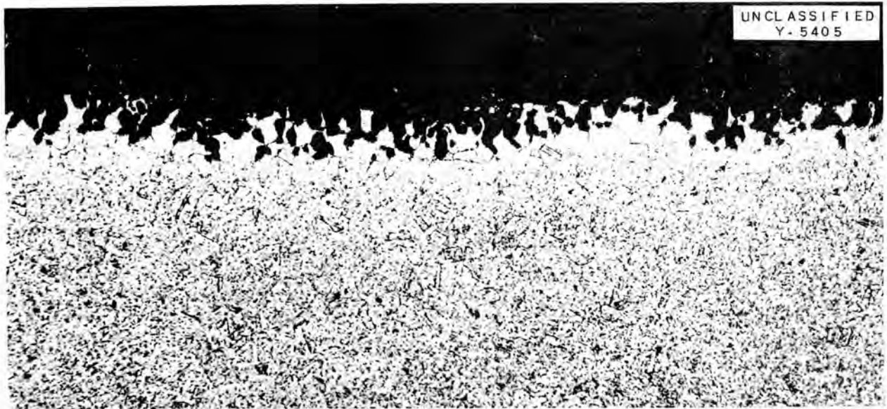
Fig. 33. Intergranular Attack of Type-310 Stainless Steel Tested in 44% Lead-56% Bismuth Alloy for 100 hr at 1500°F. 200X.
