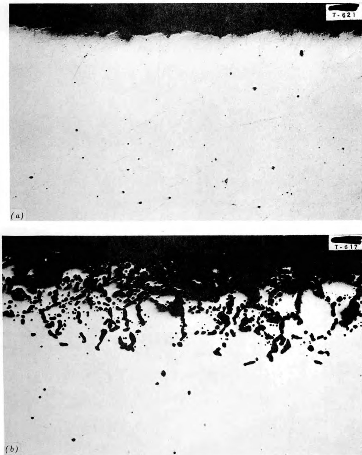
Fig. 37. Sections of Hot and Cold Legs of a Type-316 Stainless Steel Convection Loop After Circulating the Fluoride Fuel ( \text{NaF-KF-LiF-UF}_4 ) for 123 Hours. (a) Cold leg section, <1250^\circ\text{F} . 250X. (b) Hot leg section, 70 hr at 1500^\circ\text{F} , 63 hr at 1600^\circ\text{F} . 250X.
