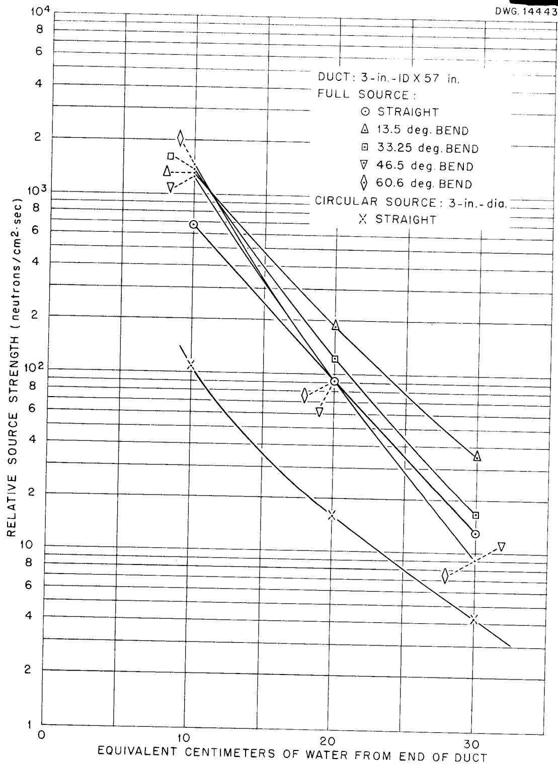
Fig. 28. Comparison of Relative Source Strengths ( n_0 ) from Various Geometries of the 3-in. Duct.
