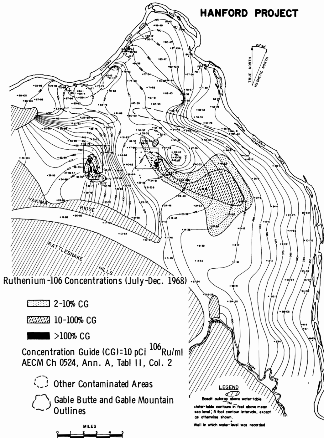
FIGURE 1. Ruthenium-106 Concentrations Beneath the Hanford Project
