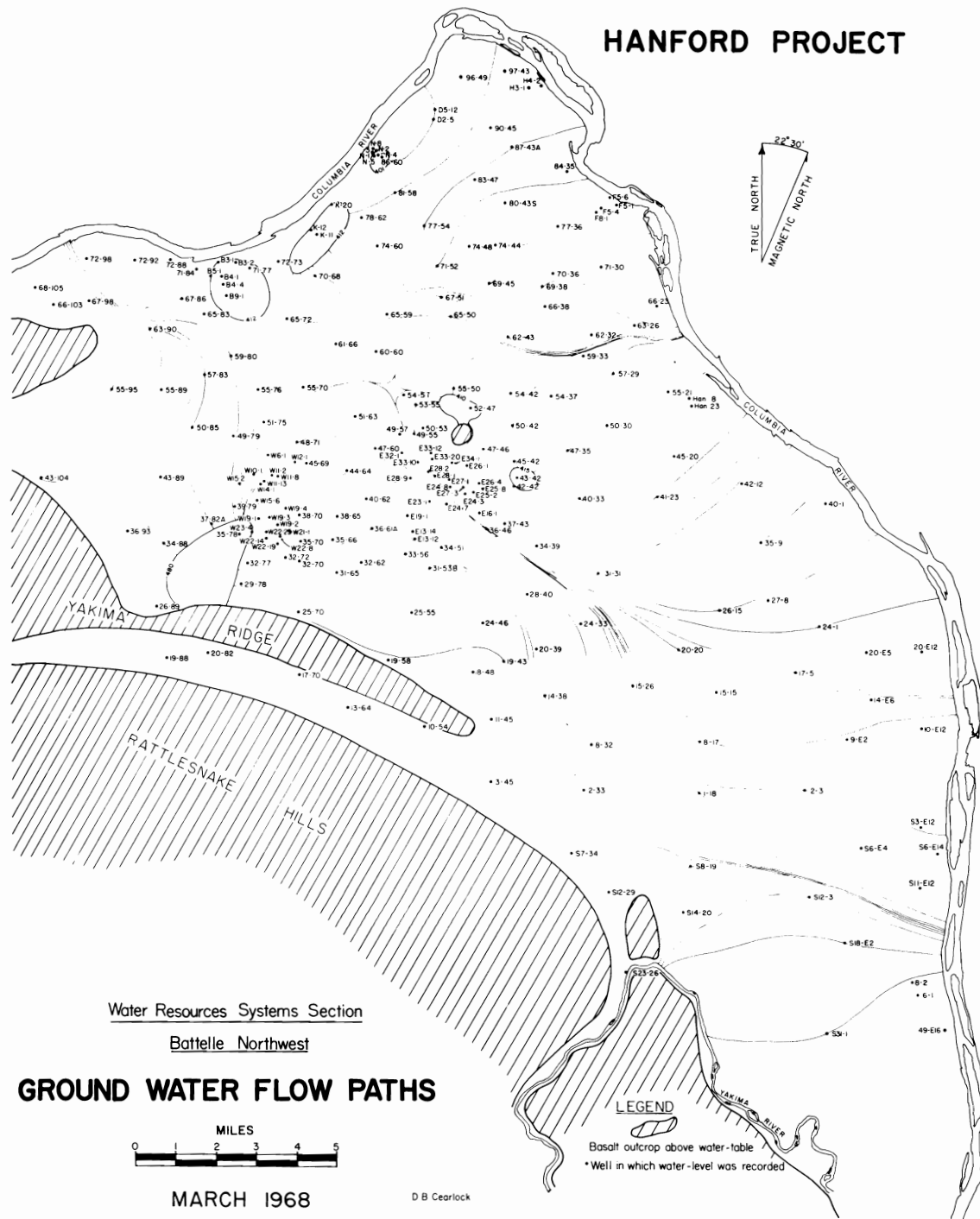
FIGURE 3. Ground-Water Flow Paths (Toward the Columbia River) Beneath the Hanford Project
